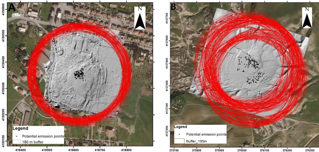
897 Fig.6. Buffer circumferences in ArcGIS 10.5 at Santa Barbara (A) and Aragona (B) mud volcanoes areas. (Source: 898 2017 DSM's in ArcGIS 10.5).
