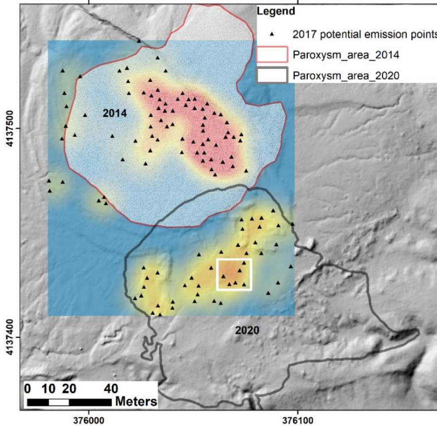
1026 Fig. 9 , Density maps for the 2017 emission points (Red: High density; yellow: low density). The covered surface area for 1027 the 2014 and 2020 paroxysms is shown with red and grey lines , respectively. In the white square, the 2017 emission 1028 points, likely responsible for the new 2020 paroxysm event. (Source: 2017 DTM's in ArcGIS 10.5) 1029 1030
