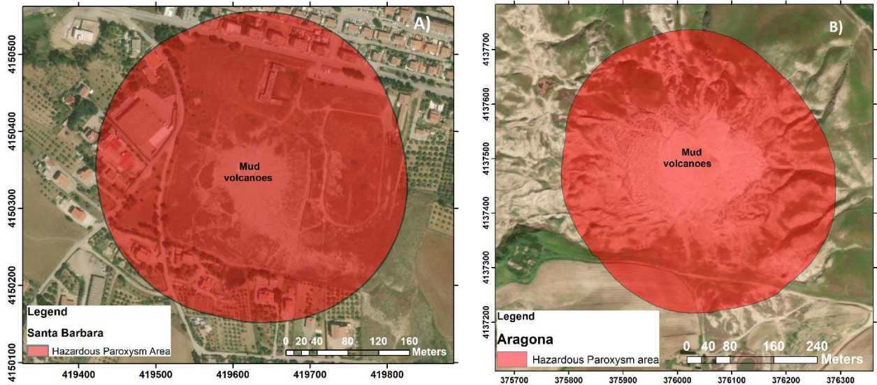
965 Fig. 7. Hazardous Paroxysm areas in ArcGis 10.5 for Santa Barbara (A) and Aragona (B) mud volcanoes area. (Source 966 image from ArcGIS 10.5, ESRI)
