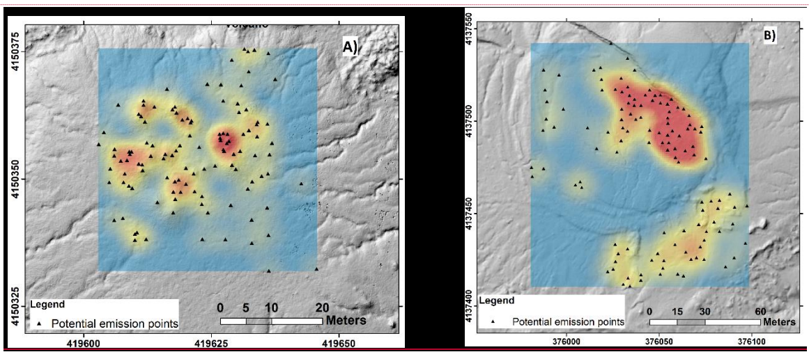
Fig.5. Density maps of the potential emission points investigated. Red: high-density values; Yellow: low-density values. A) Santa Barbara MV area and at B) Maccalube of Aragona. (Source: 2017 DSM's in ArcGIS 10.5)
