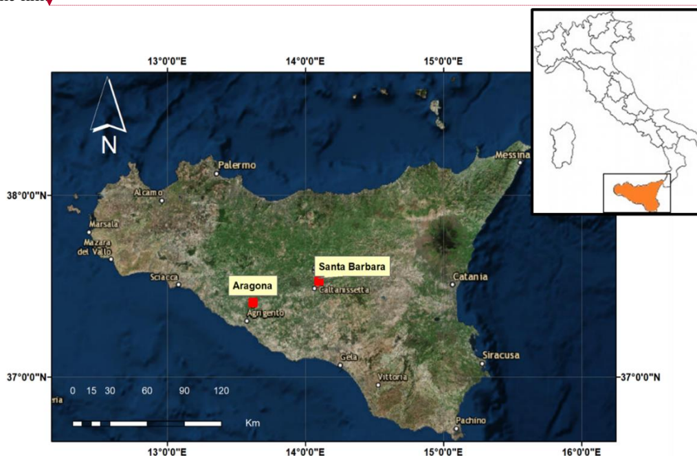
326 Fig.1. Location of the two investigated mud volcanoes areas: Santa Barbara (Caltanissetta Province) and Aragona 327 (Agrigento Province) (image from ESRI).
