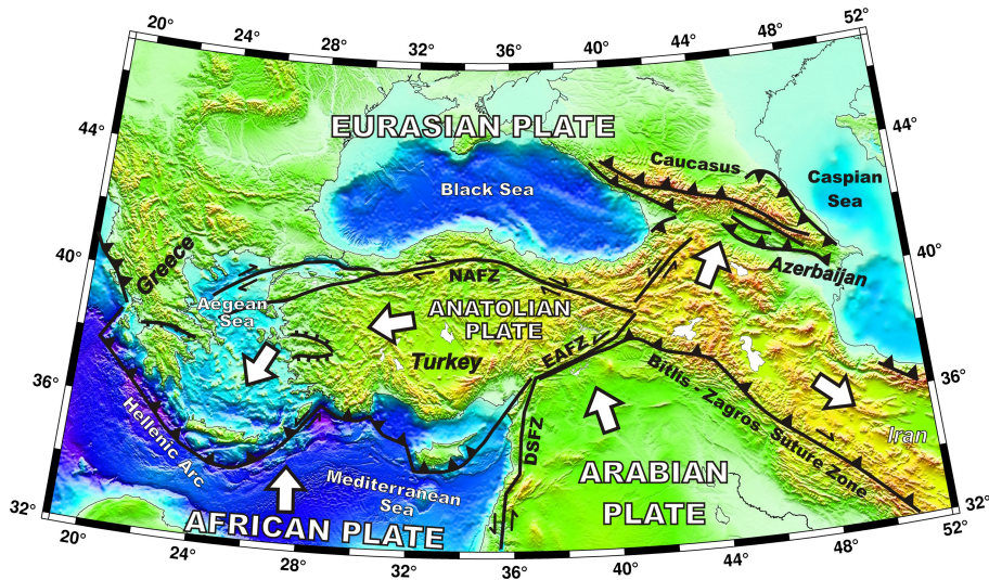
70 Figure 1. Simplified tectonic map of the Eastern Mediterranean. DSFZ: Dead Sea Fault Zone, EAFZ: East Anatolian Fault Zone, NAFZ: North Anatolian Fault Zone. Triangles indicate the direction of vergence or subduction. Bars are the down-thrown side of normal faults. White arrows are relative plate motions. The relief model is generated with the ETOPO1 model (Amante and Eakins, 2009).
