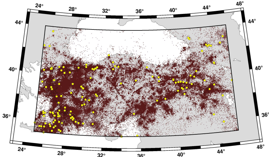
Figure 3. The earthquakes in the homogenised catalogue (dots). Yellow circles are the events with an equivalent moment magnitude ( M_w^* ) greater than 6.0 (total, 145 events).
