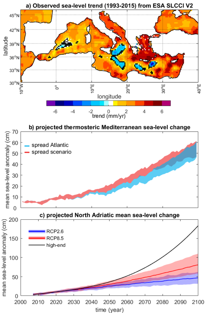
1580 Figure 7: Observed and projected trends of Mediterranean sea-level variations. (a) Sea-level trends in the Mediterranean Sea 1585 obtained using the ESA SLCCI V2 product over the period 1993-2015. Dots indicate grid points where the trend is not different from zero within the associated error range, estimated as the 90% confidence interval from linear least-squares regression analysis. (b) Projected thermosteric basin-average sea-level anomalies for the Mediterranean Sea and associated uncertainties related to the Atlantic hydrographic boundary conditions (blue) and to the socio-economic scenarios based on the Special Report on Emissions Scenarios (red) with the regional ocean model NEMOMED8, for the 2000-2100 period (vs. 1961-1990). Uncertainties are the spread among the simulations with only differing Atlantic boundary conditions (blue) and the spread among the simulations with differing socio-economic scenarios (red). Adapted from Slangen et al. (2016). (c) Projected Northern Adriatic RSL anomalies and associated uncertainties related to socio-economic scenarios (shading: 5-95 percentile range, line: median). See main text for details on the calculation of uncertainties. Adapted from Thiéblemont et al. (2019).
