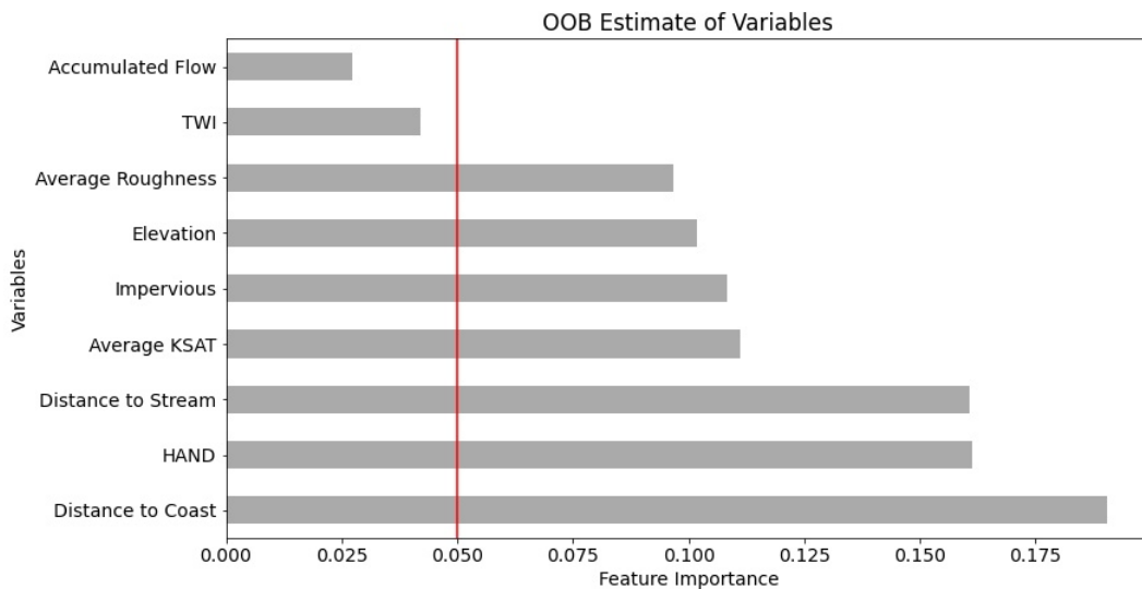
Figure 3. Feature importance chart. Note variables below, 0.05 were removed from the final model. The red line denotes the cutoff value for the final model.
