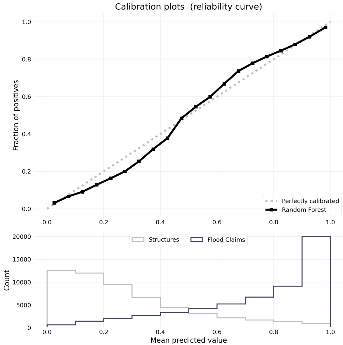
Figure 5. Calibration plot (top) with histogram of flooded / non-flooded samples and their predicted values.
