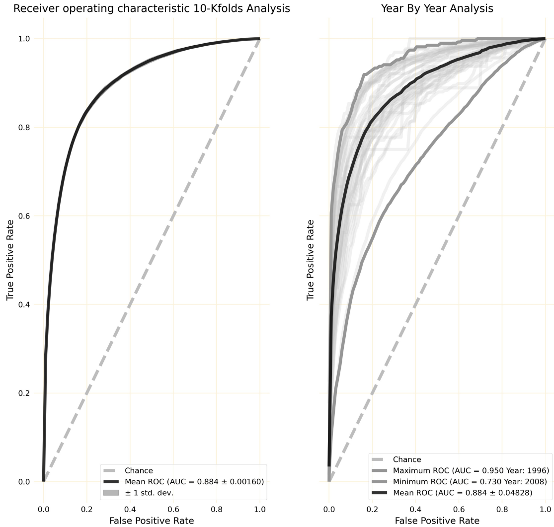
Figure 4. Left) The Receiver Operating Characteristic (ROC) shown for 10k-folds cross validation. Right) The ROC shown for the year-by-year analysis. The year by year analysis shows generalizability of the model by predicting how well a standalone years flooding will fit within the model. This approach also identifies years with storm outliers.
