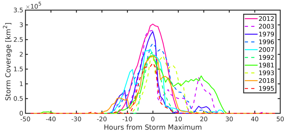
385 Figure 3. Spatial extent of the windstorms measured in \text{km}^2 over the Northeastern states relative to t_p . The spatial extent is 390 described as the area of ERA5 grid cells wherein the U > U_{999} . Values are shown for 48 hours preceding and following each 395 windstorm peak.
