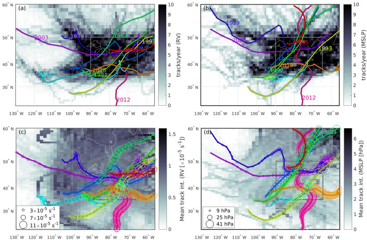
Figure 6. Cyclone tracks associated with each of the top 10 windstorms (individual colors) plotted over a heat map of cyclone densities for (a) relative vorticity (RV) and (b) mean sea level pressure (MSLP). Cyclone intensities for analyses of (c) 700 hPa RV and (d) MSLP (shown as an absolute value) for each of the top 10 windstorms (where the symbol diameter scales with intensity) plotted over a heat map of mean cyclone intensities. Symbol sizes shown in the figure legends represent the 10th, 50th and 90th percentile cyclone intensities from among the top 10 windstorms. Track densities and intensities in all four panels are computed at the ERA5 grid resolution and then averaged to a 1^\circ \times 1^\circ grid to aid legibility. These background field values include only cyclones that track into the Northeast rectangle (shown in grey) during cold months (October-April 1979-2018) and are anomalies identified in the filtered fields, obtained from the spectral filtering which has the large-scale background removed for the tracking. Color coding of the cyclone tracks associated with each windstorm is as in Fig. 3.
