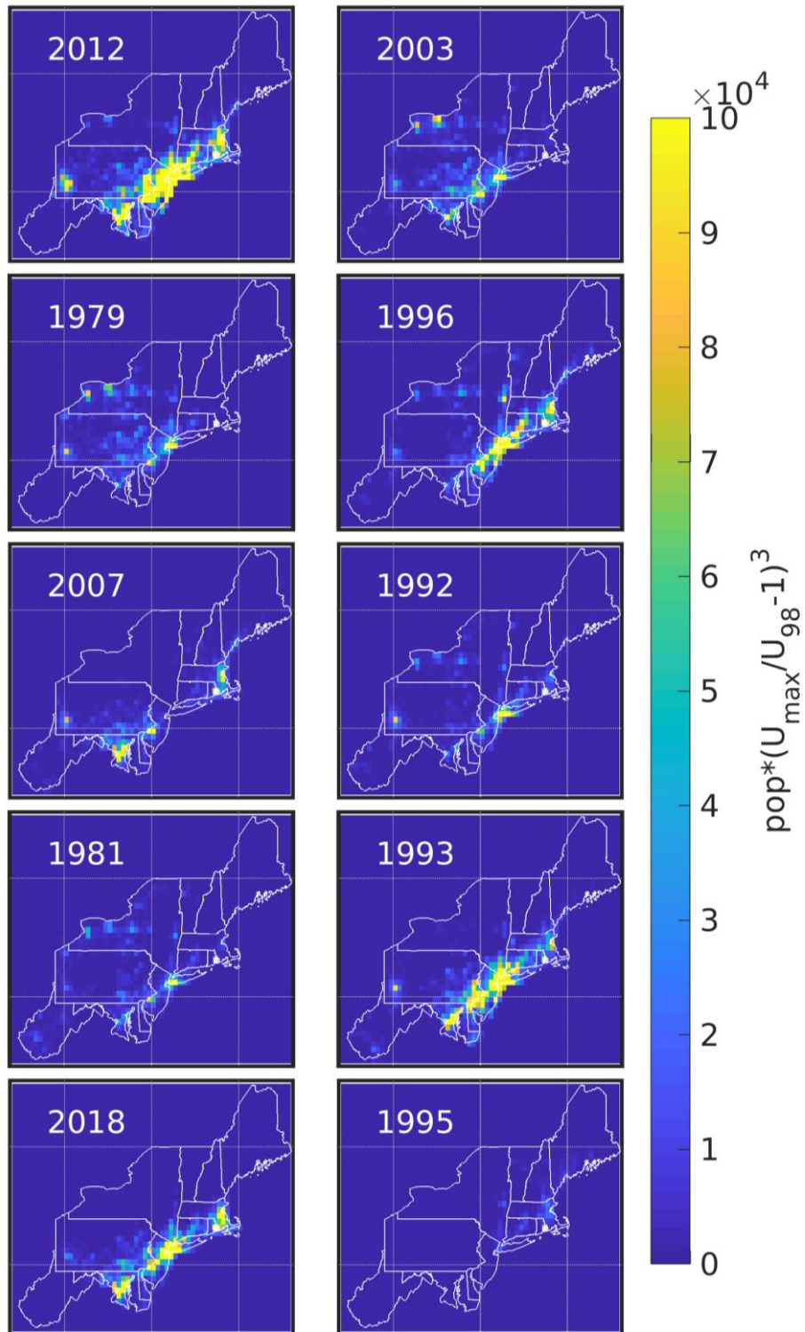
535 Figure 8. Contribution to the loss index (LI; Equation 4) from each ERA5 grid cell associated with each windstorm. Northeastern state borders and coastlines (Atlantic Ocean and Great Lakes) are shown in white.
