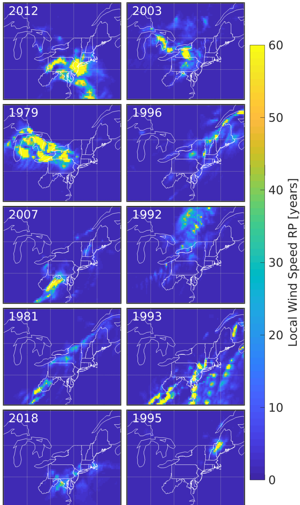
Figure 7. Return period (in years) of storm-maximum wind speed ( U_{peak} ) in each ERA5 grid cell associated with each windstorm. The color scale is truncated at 60 years for legibility. But, for example, the RP of the maximum wind speeds at 100 m during Hurricane Sandy (2012) exceeds 100 years for multiple grid cells. Northeastern state borders and coastlines (Atlantic Ocean and Great Lakes) are shown in white.
