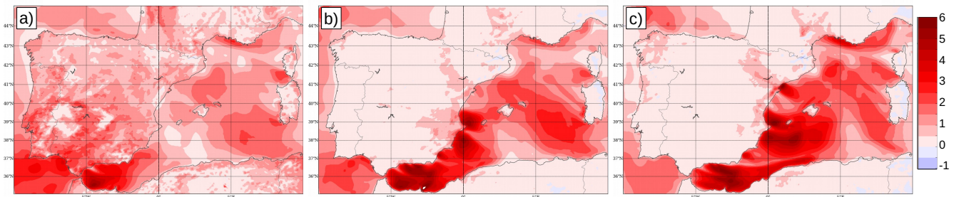
Figure 4. 6-hour cumulative surface evaporation ( \text{kg m}^{-2} ) from successive ARPEGE forecasts: (a) at 18:00 UTC on 14 October (forecast basis: 14 October 12:00 UTC), (b) at 00:00 UTC on 15 October (forecast basis: 14 October 18:00 UTC), and (c) at 06:00 UTC on 15 October (forecast basis: 15 October 00:00 UTC).
