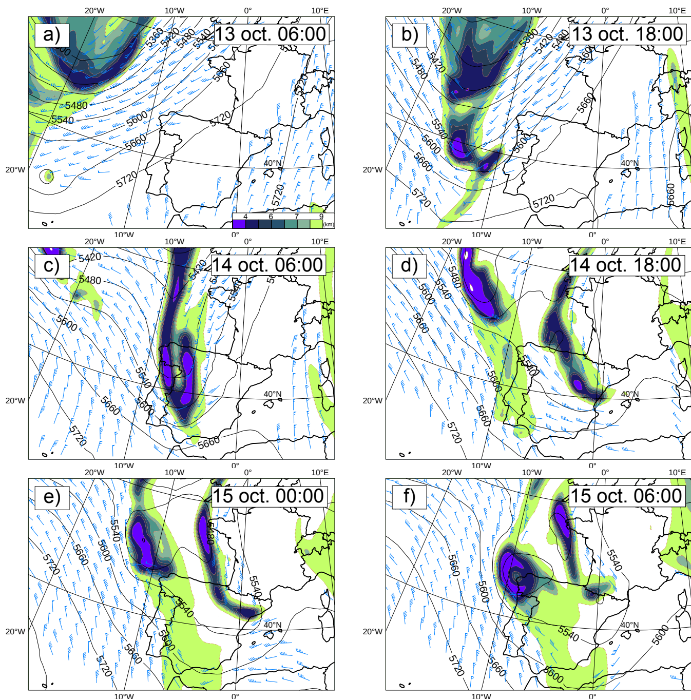
Figure 2. Same as Fig. 1 but for geopotential height at 500 hPa (solid lines, gpm), geopotential height (coloured areas, gpk) and horizontal winds (barbs, m s -1 ) along the 2 PVU surface.
