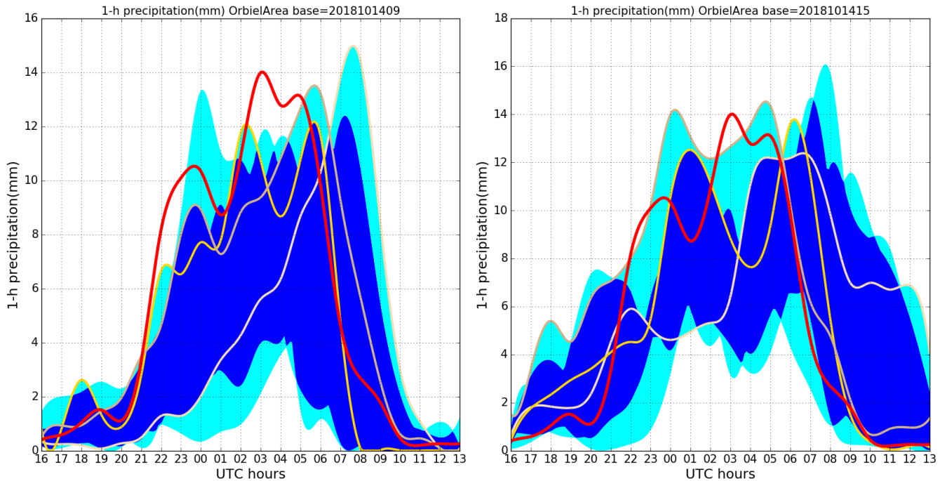
Figure 8. Time series of hourly precipitation over the area of interest (depicted in red in Fig. 6). Left and right panels, respectively: AROME-EPS forecasts based on the 09:00 and 15:00 UTC analyses on 14 October. Red curve: SWS ANTILOPE observation. Yellow: forecasts from three rainiest members of each ensemble. Light blue area: ensemble minimum and maximum forecasts. Dark blue areas: interval between the 15 % and 85 % percentiles.
