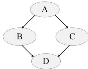
Figure 6. Diagrammatic depiction of Bayesian model
