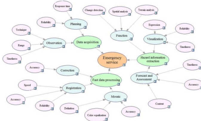
Figure 8. BN topology of service capacity evaluation mode
