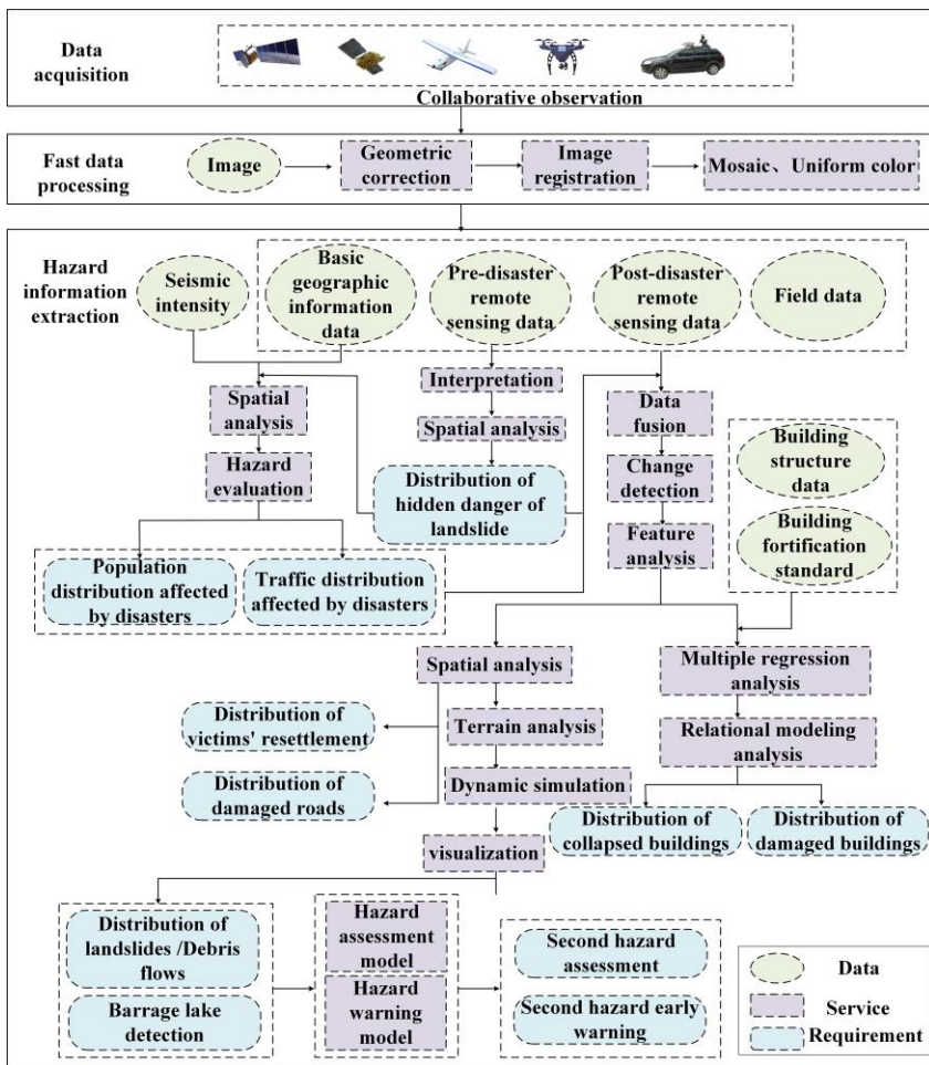
Figure 7. Earthquake-remote sensing emergency response service chain
