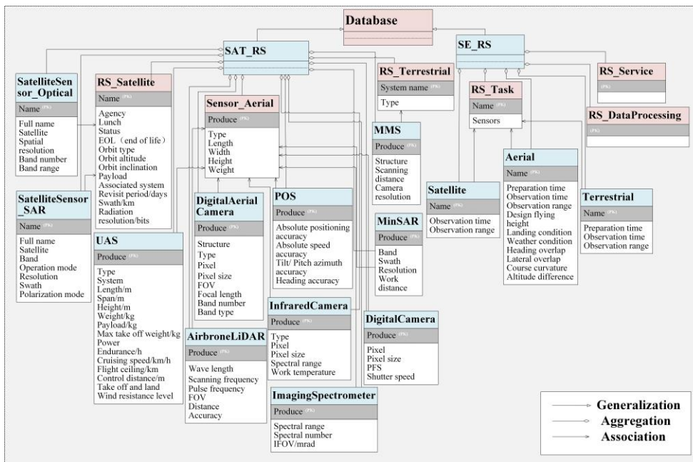
Figure 3. Unified Modeling Language (UML) of database
