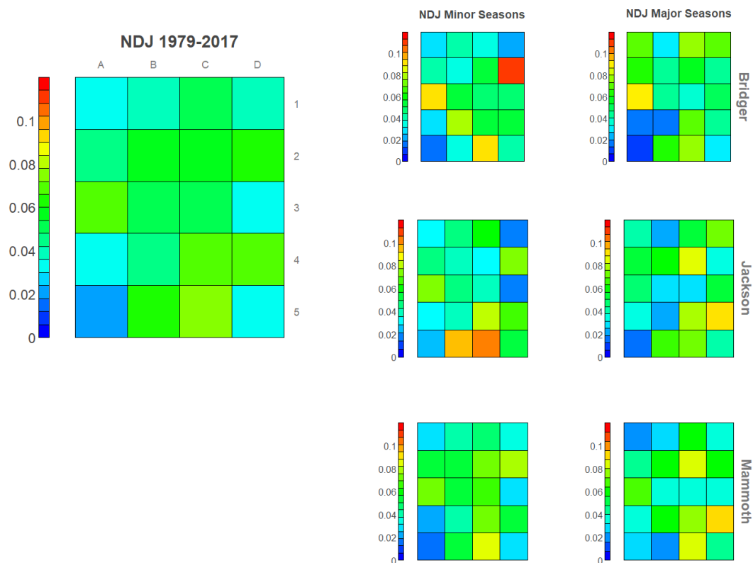
805 Figure 5: Relative frequencies for each synoptic type from November-January for the entire study period (upper left), over all minor seasons (left column), and all major seasons (right column). Heat maps are given for Bridger Bowl (top row), Jackson (center row), and Mammoth Mountain (lower row). Frequencies are calculated by summing counts of days assigned to each synoptic type over all major (minor) seasons and dividing by total number of days for all major (minor) seasons.
