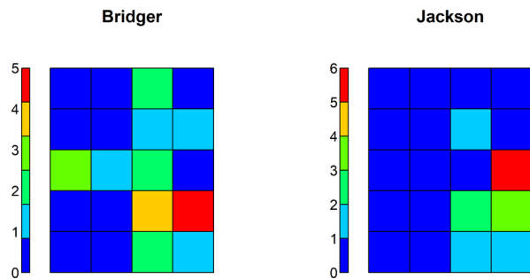
815 Figure 7: Counts for each synoptic type within the 72 hours prior to deep wet slab avalanches at Bridger Bowl (left) and the Jackson area (right).
