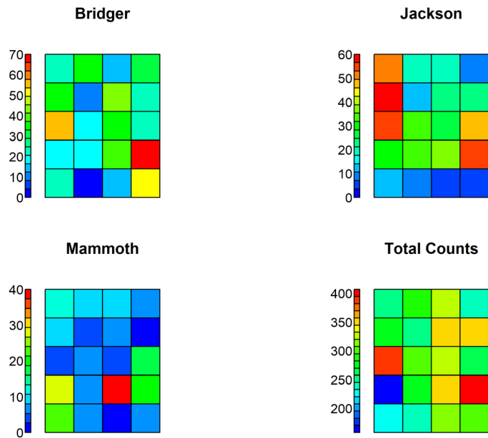
810 Figure 6: Relative frequencies for each synoptic type within 72 hours prior to a day with dry deep slab avalanches recorded at Bridger Bowl (upper left), Jackson Hole (upper right), Mammoth Mountain (lower left), and total counts for the duration of the study period.
