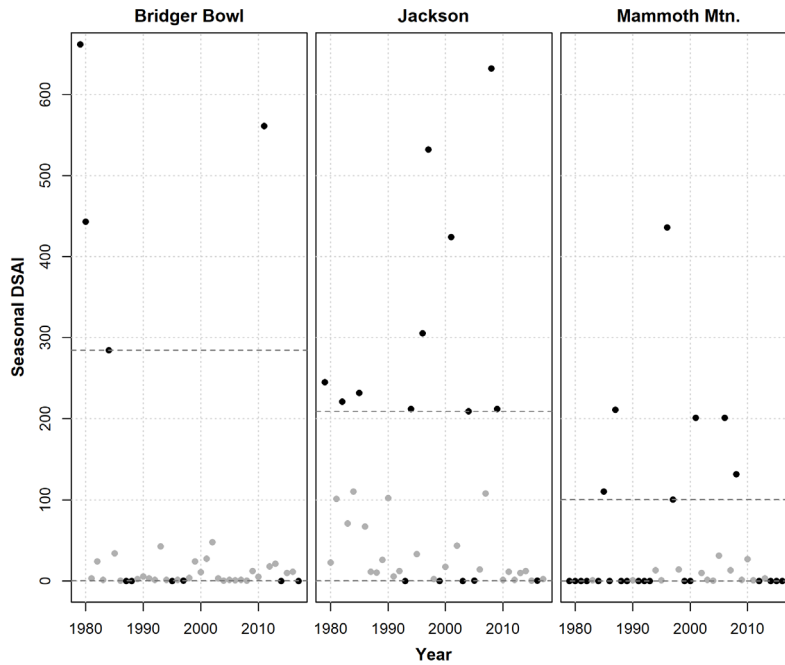
800 Figure 4: Scatterplots of seasonal deep slab activity index scores for Bridger Bowl, MT (left), Jackson Hole (center), and Mammoth Mountain, CA (right). Highlighted points represent the years considered as major and minor deep persistent avalanche seasons, and dashed lines represent the cutoff thresholds used to identify those points.
