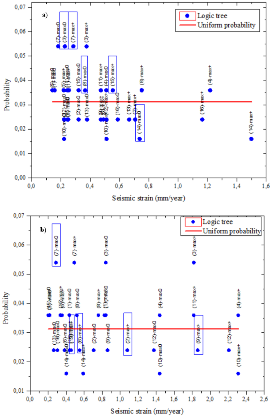
440 Figure 7: Seismic strain and probability for each of the 32 models that result from the logic tree proposal of Vilanova and Fonseca (2007). The scenarios outlined are the ones chosen to be tested with neotectonics modelling. a) the LTV source zone. b) the 1755 source zone.
