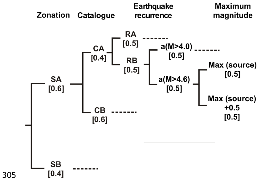
Figure 4: Logic tree used for hazard calculation. The weight of each branch is shown in straight parentheses (modified from Vilanova and Fonseca, 2007).
