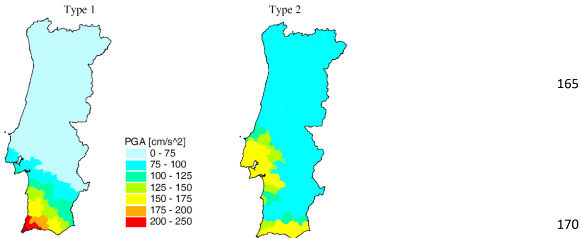
Figure 2: Seismic hazard maps expressed as Peak Ground Acceleration (PGA) expected to be exceeded in 50 years with 10% probability. (a) From the ESHM13 model by Woessner et al. (2015), units in g; (b) From the PSHA study used in Portugal for the revision of the building codes according to EC8 guidelines (Campos Costa et al., 2008), units in \text{cm/s}^2 . Type 1 refers to a “far” (offshore) source while type 2 refers to a “near” source. These maps show the inconsistency of PSHA models, as two options for the chosen models.
