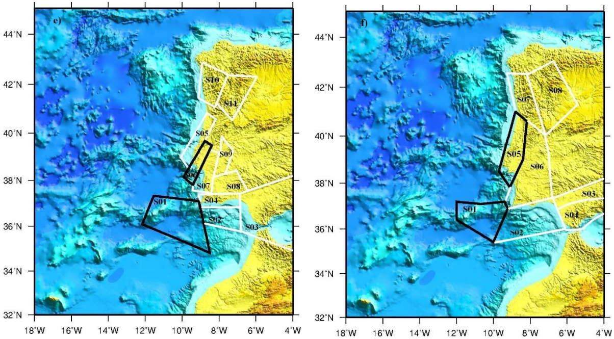
180 Figure 3 (continued): Seismogenic zones proposed for the 5 PSHA studies analysed in this work.
