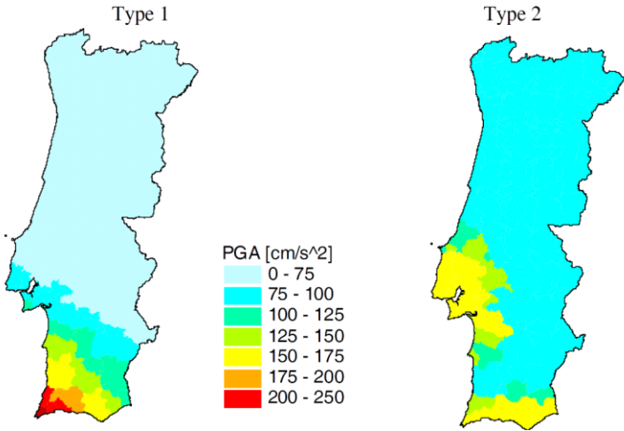
155 Figure 2: Seismic hazard maps expressed as Peak Ground Acceleration (PGA) expected to be exceeded in 50 years with 10% probability. (a) From the ESHM13 model by Woessner et al. (2015), units in g; (b) From the PSHA study used in Portugal for the revision of the building codes according to EC8 guidelines (Campos Costa et al., 2008), units in \text{cm/s}^2 . Type 1 refers to a “far” (offshore) source while type 2 refers to a “near” source. These maps show the inconsistency of PSHA models, as two options for the chosen models.
