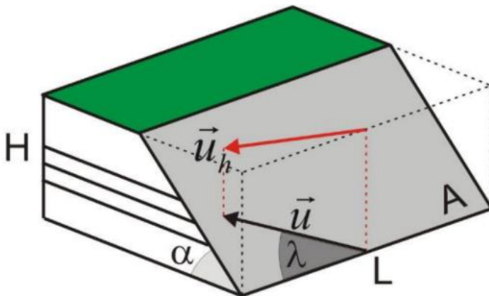
Figure 5: Simple earthquake generation model used to calculate the seismic strain rate. Being, A the area of the fault; L the length of the 375 fault; H the thickness of the seismogenic layer and \alpha the dip of fault (Matias and Teves-Costa, 2011a, b).
