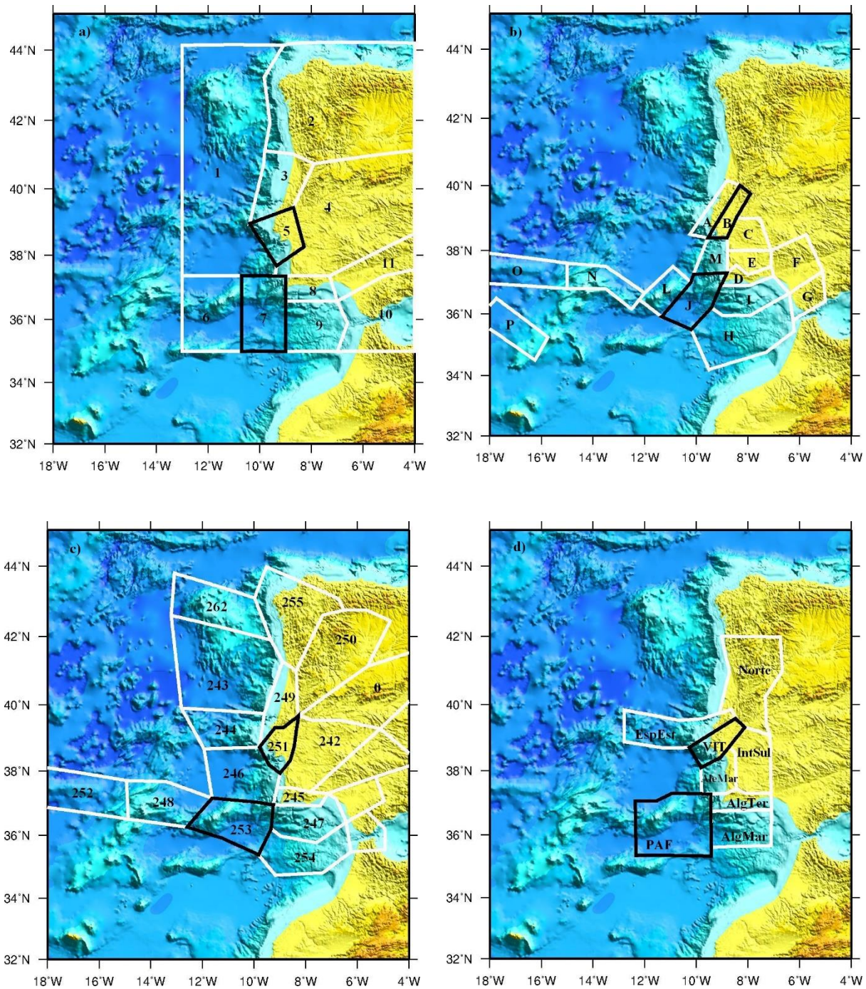
185 Figure 3: Seismogenic zones proposed for the 5 PSHA studies analysed in this work. The zones corresponding to Lower Tagus Valley (LTV) sources and 1755 earthquake selected for sanity check are outlined in black. a) the National Annexes of Eurocode 8 (EC8), adapted from Campos Costa et al. (2008). b) the ERSTA study, adapted from Carrilho et al. (2010). c) the SHARE study, adapted from Woessner et
