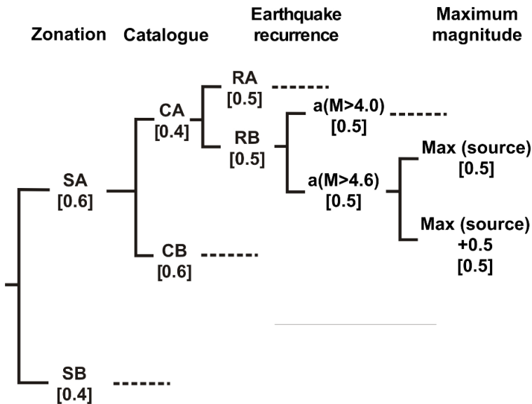
300 Figure 4: Logic tree used for hazard calculation. The weight of each branch is shown in straight parentheses (modified from Vilanova and Fonseca, 2007).
