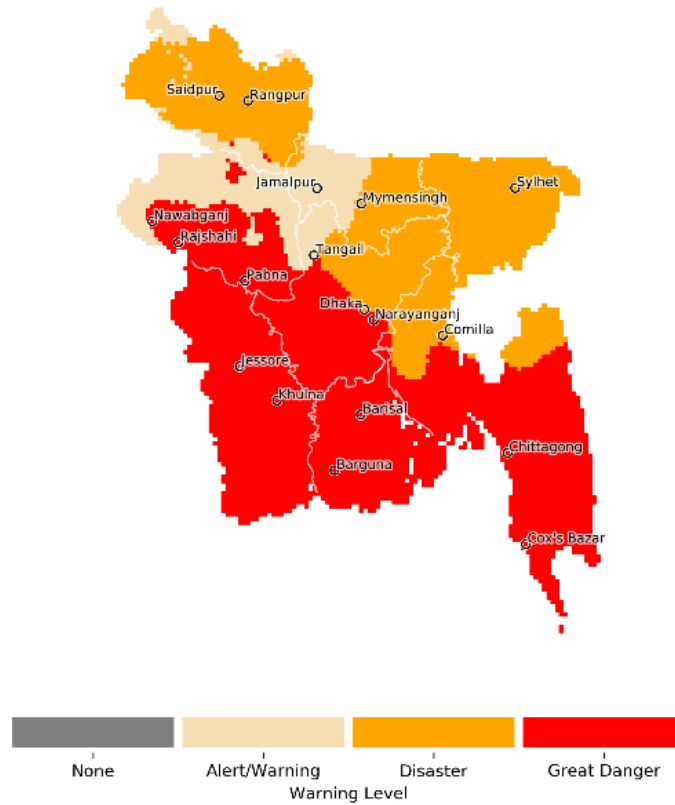
405 Figure 6: Example warning status given an impending landfalling tropical cyclone over Bangladesh. These warnings represent the most effective action minimising the loss as defined in Table 1.
