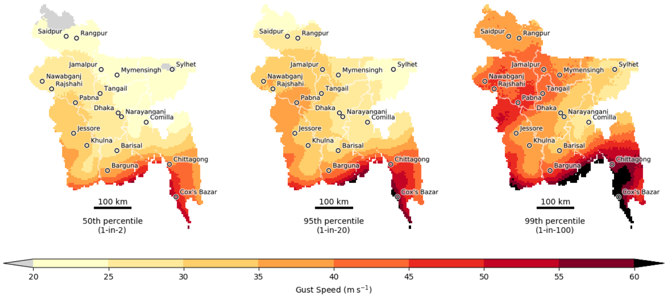
385 Figure 3: Gust speed exceedance thresholds for the 50 th (left) 95 th (middle) and 99 th (right) percentile credible intervals. The 50 th , 95 th and 99 th percentiles represent the maximum gust speeds expected from a 1-in-2, 1-in-20 and 1-in-100 event respectively (conditional on a tropical cyclone making landfall over Bangladesh). These credible intervals are based on the posterior model distribution derived from all 12 named tropical cyclones, conditional on a tropical cyclone making landfall in Bangladesh. The 20 – 60 \text{m s}^{-1} gust speed range roughly corresponds to a range of 39 – 117 kn, equivalent to the cyclonic to super cyclonic storm classification used in Bangladesh. Province boundaries are outlined in white, with the 18 most populated towns and cities marked by circles.
