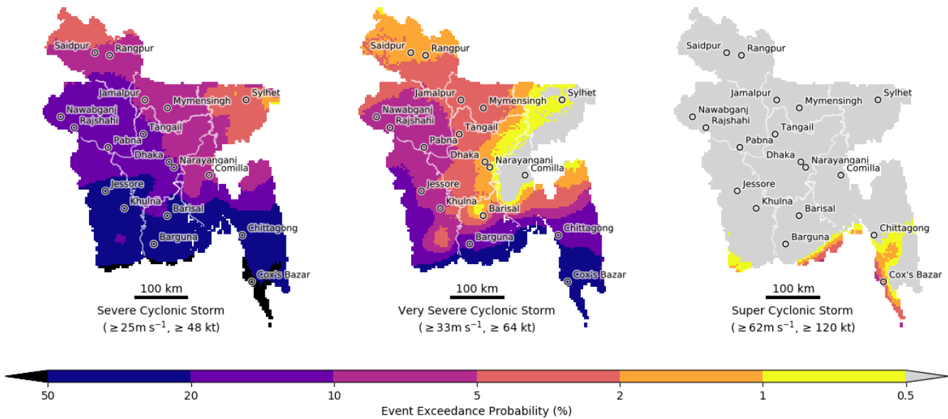
395 Figure 4: Event exceedance probabilities for a severe cyclonic storm (left), very severe cyclonic storm (middle) and super cyclonic storm (right) WMO tropical cyclone classifications used in the Bay of Bengal (WMO, 2018). Event exceedance probabilities show the likelihood of a maximum tropical cyclone gust speed being greater than or equal to the corresponding classification wind threshold, conditional on a tropical cyclone making landfall over Bangladesh. An exceedance threshold of 50% (0.5%) represent a 1-in-2 (1-in-200) chance of a tropical cyclone exceeding a given threshold. Areas where the exceedance probability is > 50\% ( < 0.5\% ) are shaded black (grey). Province boundaries are outlined in white, with the 18 most populated towns and cities marked by circles.
