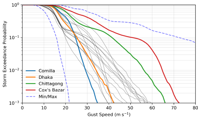
400 Figure 5: Exceedance probability curves for 18 of the most populated towns and cities in Bangladesh (grey lines), with 4 key cities highlighted: Dhaka (orange), Comilla (blue), Chittagong (green) and Cox's Bazar (red). For reference, the minimum and maximum range of exceedance probabilities (across all of Bangladesh) are represented by the dashed lines. Note that storm exceedance probability is shown on a log-scale.
