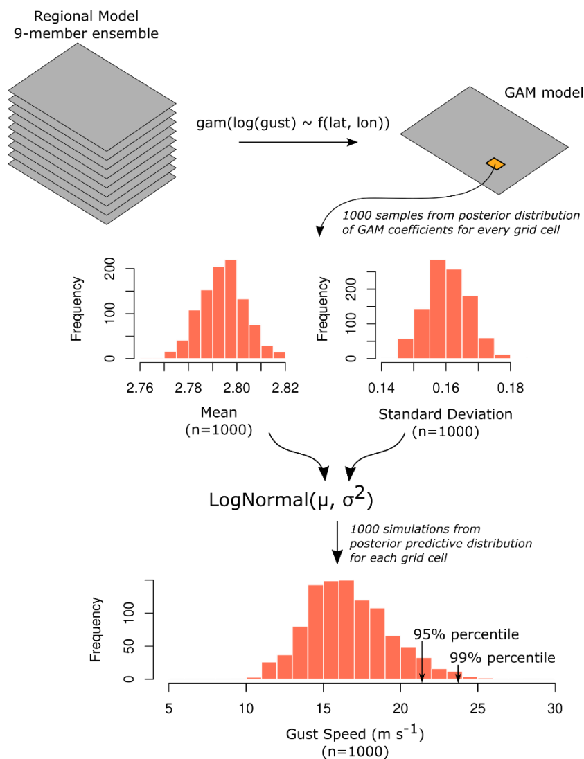
385 Figure 1 Summary of generalised additive modelling and the derivation of the posterior prediction gust speed distribution. The posterior predictive distribution is found for each grid cell of the regional model domain. Gust speed prediction intervals are found from the percentiles of the posterior predictive distribution.
