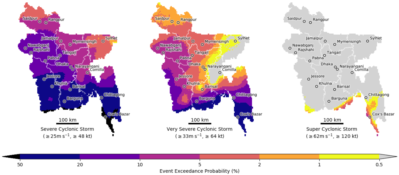
400 Figure 4: Event exceedance probabilities for a severe cyclonic storm (left), very severe cyclonic storm (middle) and super cyclonic storm (right) WMO tropical cyclone classifications used in the Bay of Bengal (WMO, 2018). Event exceedance probabilities show the likelihood of a maximum tropical cyclone gust speed being greater than or equal to the corresponding classification wind threshold, conditional on a tropical cyclone making landfall over Bangladesh. An exceedance threshold of 50% (0.5%) represent a 1-in-2 (1-in-200) chance of a tropical cyclone exceeding a given threshold. Areas where the exceedance probability is > 50\% ( < 0.5\% ) are shaded black (grey). Province 405 boundaries are outlined in white, with the 18 most populated towns and cities marked by circles.
