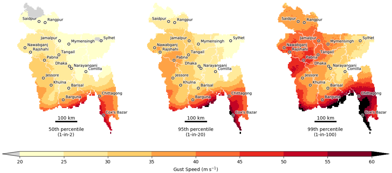
Figure 3: Gust speed exceedance thresholds for the 50 th (left), 95 th (middle) and 99 th (right) percentile credible intervals. The 50 th , 95 th and 99 th percentiles represent the maximum gust speeds expected from a 1-in-2, 1-in-20 and 1-in-100 event respectively (conditional on a tropical cyclone making landfall over Bangladesh). These credible intervals are based on the posterior model distribution derived from all 12 named tropical cyclones, conditional on a tropical cyclone making landfall in Bangladesh. The 20 – 60 m s -1 gust speed range roughly corresponds to a range of 39 – 117 kn, equivalent to the cyclonic to super cyclonic storm classification used in Bangladesh. Province boundaries are outlined in white, with the 18 most populated towns and cities marked by circles.
