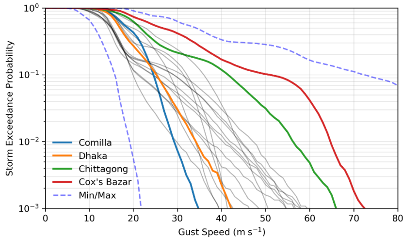
410 Figure 5: Exceedance probability curves for 18 of the most populated towns and cities in Bangladesh (grey lines), with 4 key cities highlighted: Dhaka (orange), Comilla (blue), Chittagong (green) and Cox's Bazar (red). For reference, the minimum and maximum range of exceedance probabilities (across all of Bangladesh) are represented by the dashed lines. Note that storm exceedance probability is shown on a log-scale.
