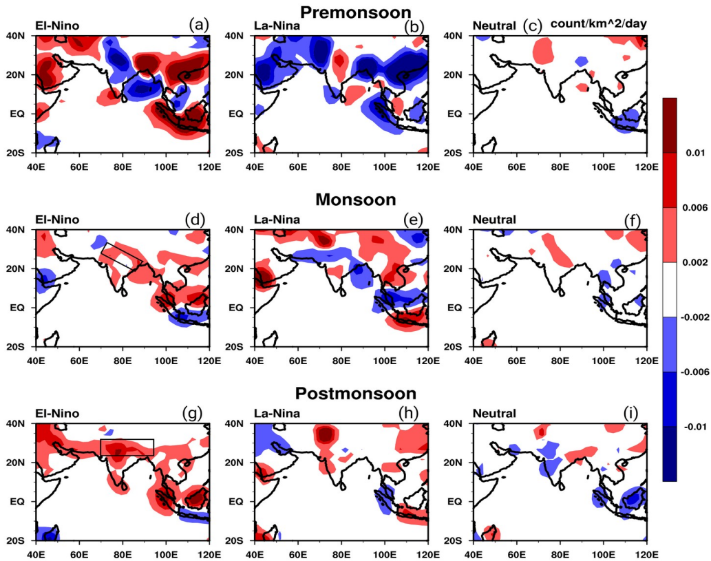
Figure 2: Anomaly composite of LFR during different ENSO phases. The box in figure (d) and (g) indicates the region of monsoon trough and western disturbance, respectively.
