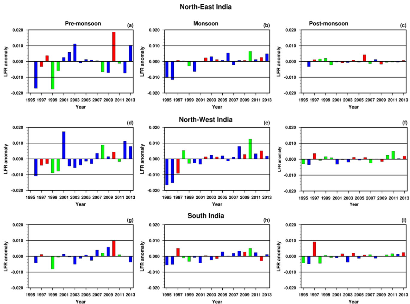
Figure 3. The anomaly of LFR during the individual years with different ENSO phases. Red color label bar corresponds to warm (El-Nino); green one corresponds to the cold (La-Nina) and blue color label bar indicates the neutral phases of ENSO
