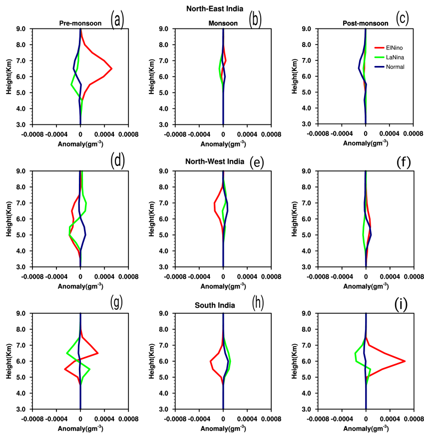
Fig. 4. Anomaly composite of graupel during different ENSO phases
