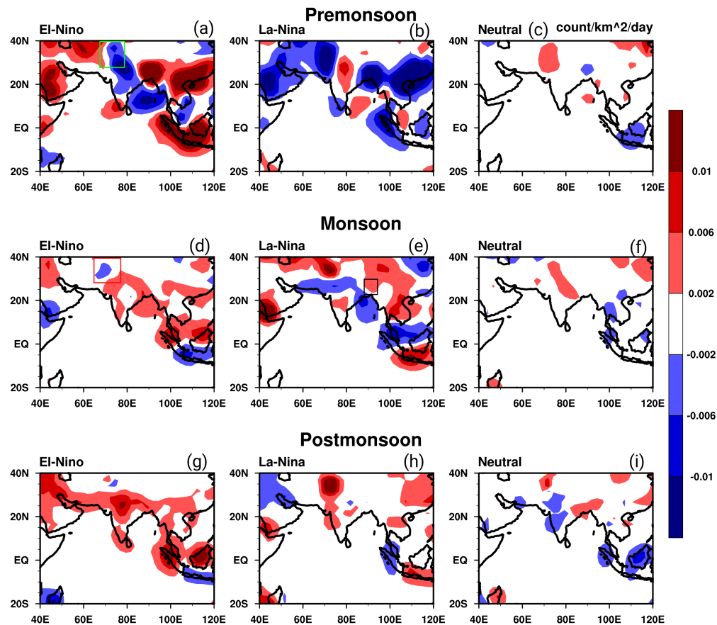
Fig. 2. Anomaly composite of LFR during different ENSO phases.
