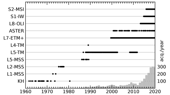
Figure 2. Temporal overview of analyzed satellite imagery. The barplot indicates the total number of available acquisitions per year.
