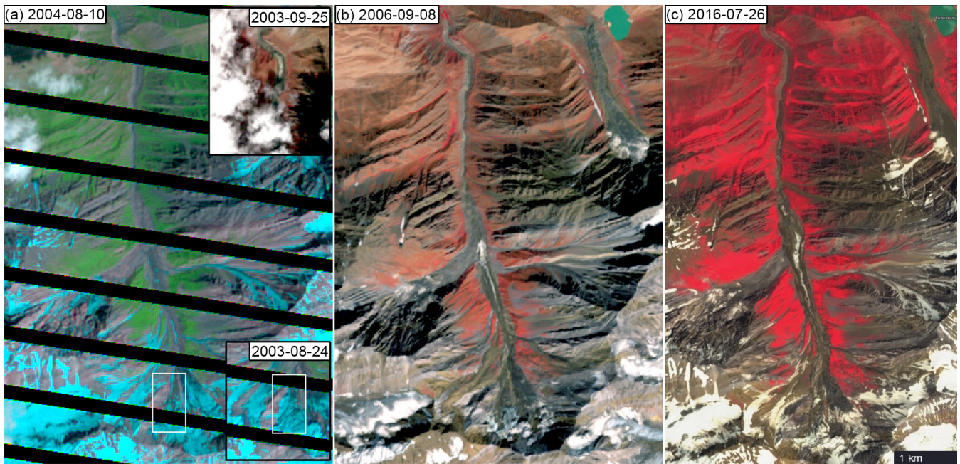
Figure A4. Mass flow events in the central Shuraki Kapali sub-catchment (a) L7 image one year after the sk-03 detachment (10 August 2004); The lower inset shows the pre-event image (24 August 2003); the ice-rich runout is shown in the upper inset (ASTER, 25 September 2003), (b) ASTER image of the ice avalanches sk-06 that broke off above the sk-03 detachment (08 September 2006). (c) S2 image of the detachment sk-16a (26 July 2016) that originated from the same location as sk-03. Landsat-7 and ASTER image courtesy of the U.S. Geological Survey. Copernicus Sentinel Data (2020).
