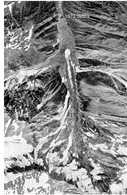
Figure A1. KH-9 image of the SK-73 rock-ice avalanche in the eastern Shuraki Kapali catchment (03 August 1973). Courtesy of the U.S. Geological survey.
