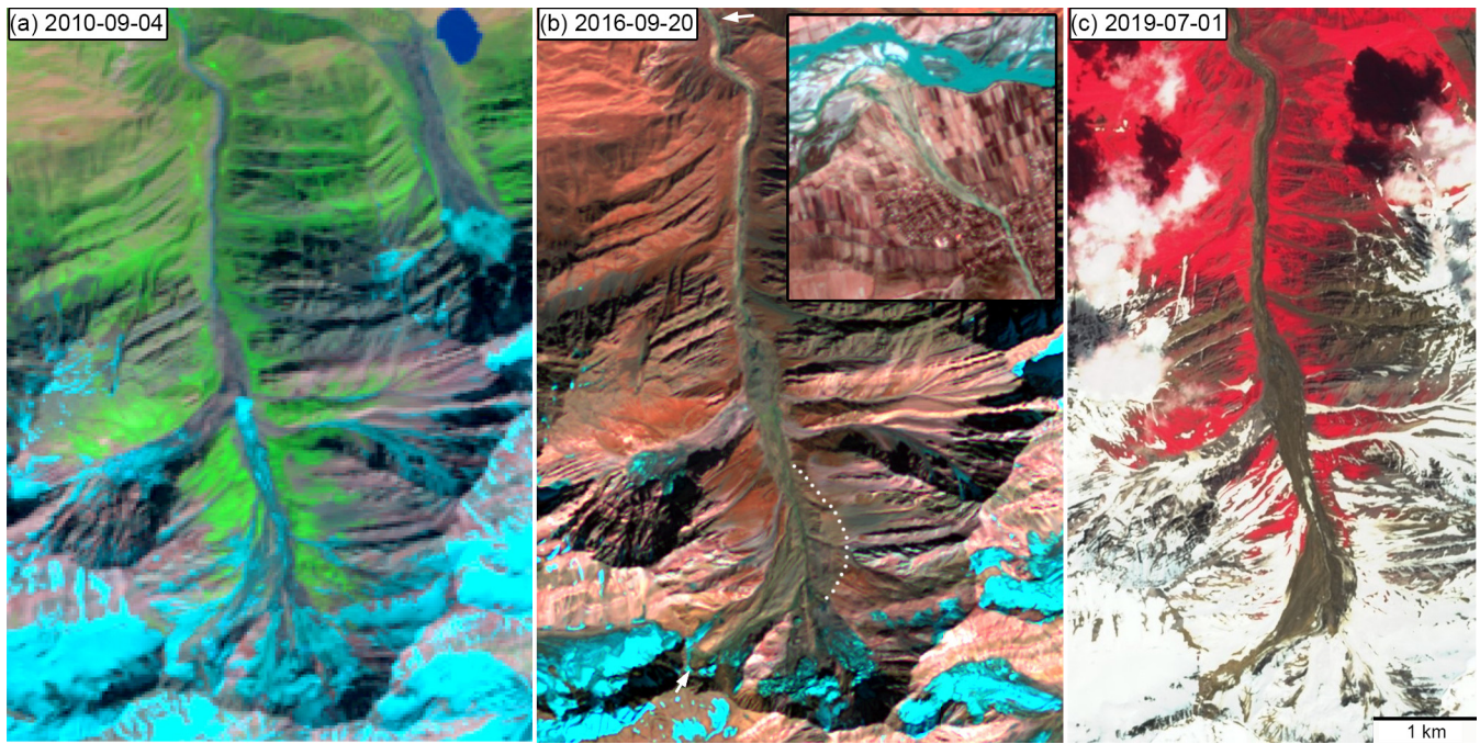
Figure A3. Mass flow events in the western Shuraki Kapali sub-catchment (continued from Fig. A2). (a) L5 image of the sk-10 rock-ice avalanche (04 September 2010); (b) L8 image of the sk-16b rock-ice avalanche (20 September 2016). The trim line of the event is indicated by dots. The arrow in the western part of the catchment indicates where the rock/ice mass detached; the arrow in the downstream valley shows where trees were removed by the resulting mass flow. The inset shows the alluvial fan 19 km downstream where a mud flow reached the Surkhob river. (c) S2 image of the sk-19 rock-ice avalanche (01 July 2019). ASTER and L8 imagery courtesy of the U.S. Geological Survey; Copernicus Sentinel Data (2020).
