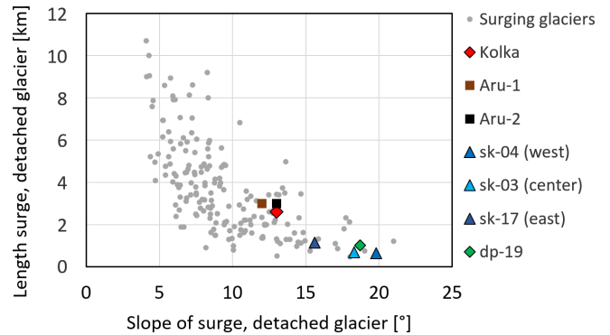
Figure 11. Horizontal length over slope of the surging part of glacier in the Pamir Mountains and surface slope of the detached parts of glacier detachments.
