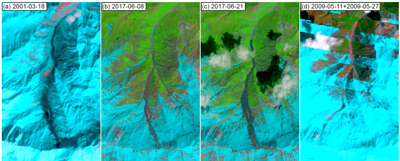
Figure A5. (a–c): rock avalanches traveling over glaciers in the eastern part of the Shikorchi catchment. (a) L7 of the shi-01 rock avalanche (18 March 2001), (b,c) S2 images of the first and second shi-17 rock avalanche (08 and 21 June 2017), (d) rock avalanche shi-09 in the western part of the catchment (image composed from two L7 images from 11 and 27 May 2009). Landsat-7 image courtesy of the U.S. Geological Survey; Copernicus Sentinel data (2020).
