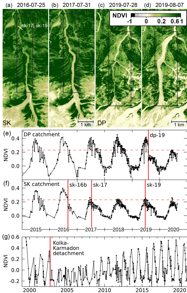
Figure 12. (a–d): NDVI before and after the sk-16b and dp-19 detachment. The white bar in (a) indicates the end of the runout of the sk-17 and sk-19 event; the sk-16b mud flow in August 2016 traveled further downstream, (e, f): NDVI time series of the mean NDVI over the eroded area (black box in a–d) of the sk-16b and dp-19 event. Vegetation hardly recovered within two years. (g): NDVI time series from the runout of the Kolka-Karmadon detachment. Vegetation recovered within about 10–15 years. Copernicus Sentinel data (2020) and Landsat-8 image courtesy of the U.S. Geological Survey.
