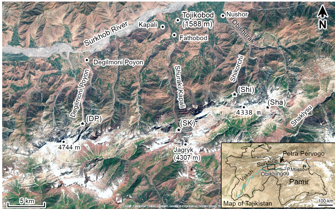
Figure 1. West Petra Pervogo range. Symbols ★ indicate catchments where large mass flows involving glacier ice occurred. Catchments are abbreviated by river names (DP, SK, Shi, Sha). Image contains Copernicus Sentinel-2 and MODIS data with borders, major rivers and place names added.
