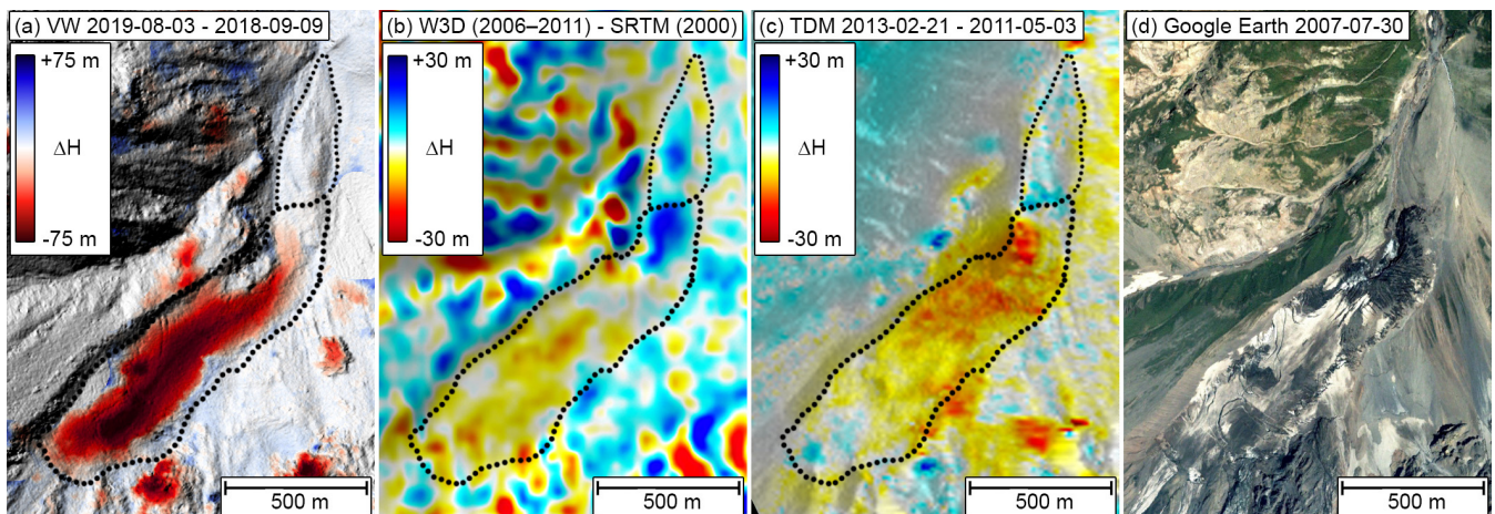
Figure 4. DEM differences of the detachment dp-19. (a): WorldView elevation differences from before and after the event reveal a detached volume of 8.6 \times 10^6 \text{ m}^3 . The shown area corresponds to the white frame indicated in Fig. 3a. (b, c) DEM differences indicate a surge-like elevation change pattern after 2000 which continued at least until 2013. (d) In 2007 strong crevassing at the glacier outline resemble surge-like dynamics. (a) 2020, DigitalGlobe; NextView License, (c) ©Google, Maxar Technologies.
