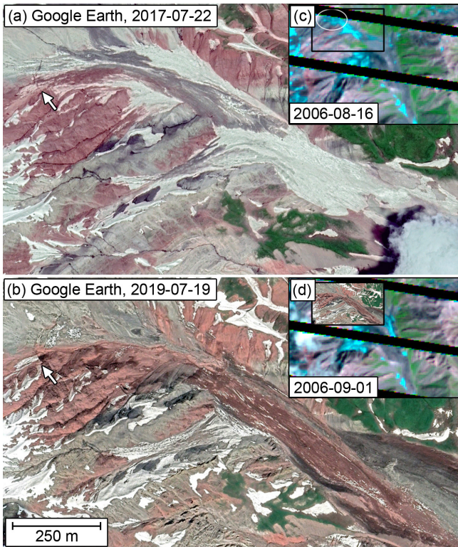
Figure 8. Imagery from before (a) and after (b) the rock-ice avalanche sha-19 that caused the disappearance of a small glacier in a side-valley of the Shaklysu river. White arrows indicate the detachment scarp. (c, d): at the same place (white circle) an earlier rock-ice avalanche (sha-06) has happened. The black box in the inset corresponds to the outline of the main images. (a, b) ©Google, Maxar Technologies. (c, d) Landsat-7 imagery courtesy of the U.S. Geological Survey.
