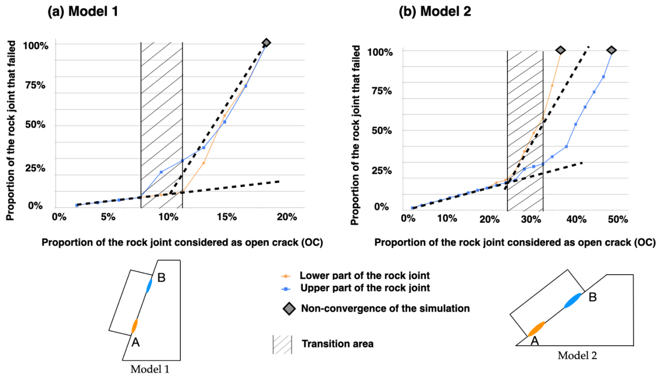
Fig. 5. Propagation of rock bridge failure for models 1 and 2 considering Scenario 2. Intentionally introduced OC are located in the upper part of the joint (blue curve) or in the lower part of the joint (orange curve). The proportion of the rock joint that failed is defined as a ratio between the number of failed contacts (OC + RBF) and the total number of contacts (OC + RB + RBF).
