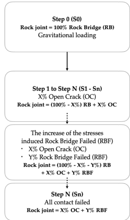
Fig. 3. Modelling process. Step 0: 100% of the rock joint is defined as Rock Bridge (RB). Step 1 to Step N: introduction of open crack (OC) along the joint. From Step 2 to Step n, it can be observed in the graph of the Model 1 the increase of shear stresses due to the introduction of OC.
