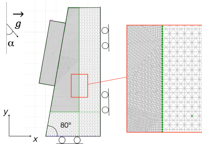
510 Fig. 2. Geometry of the both models. \alpha is equal to 0^\circ for the model 1 (slope angle: 80^\circ ) and is equal to 40^\circ for the model 2 (slope angle: 40^\circ ).
