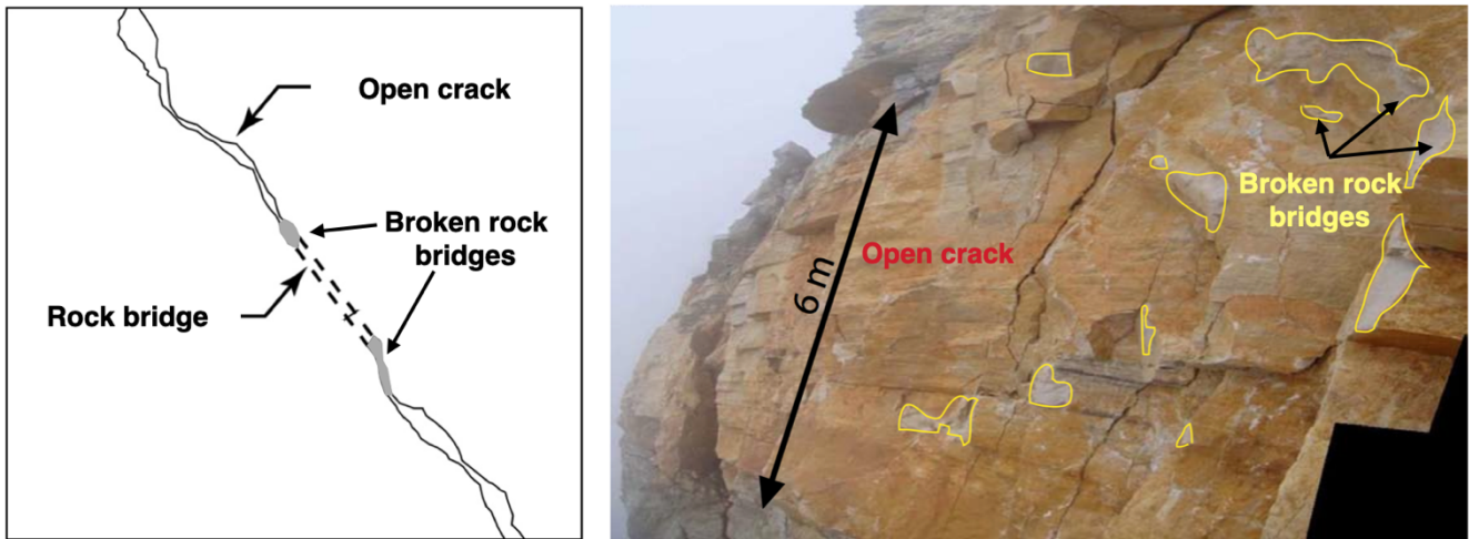
Fig. 1a (left) and b (right). Definition of rock bridges, open crack and failed rock bridges areas. Modified from Levy (Levy 2011) (with reproduction authorization).
