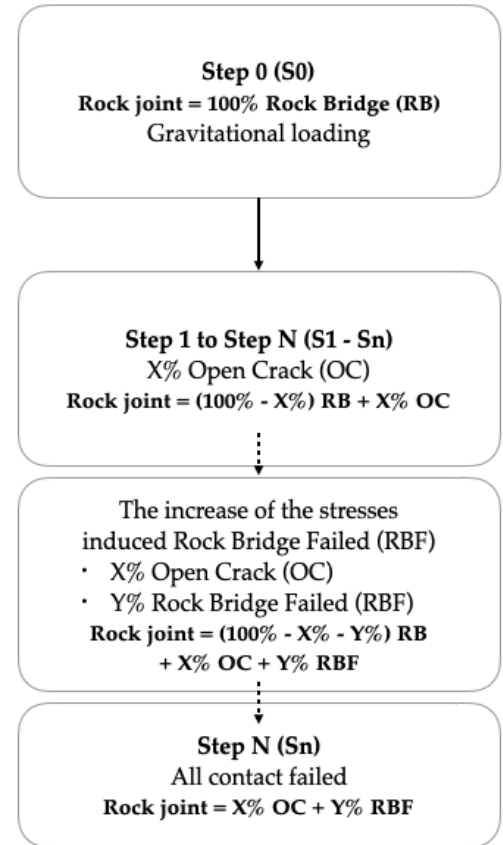
Fig. 3. Modelling process. Step 0: 100% of the rock joint is defined as Rock Bridge (RB). Step 1 to Step N: introduction of open crack (OC) along the joint. From Step 2 to Step n, it can be observed in the graph of the Model 1 the increase of shear stresses due to the introduction of OC.
