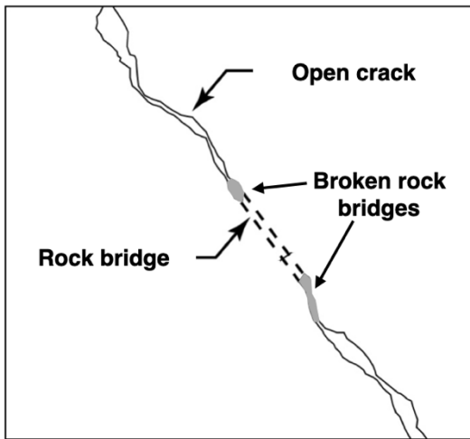
Fig. 1a (left) and b (right). Definition of rock bridges, open crack and failed rock bridges areas. Modified from Levy (Levy 2011) (with reproduction authorization).
