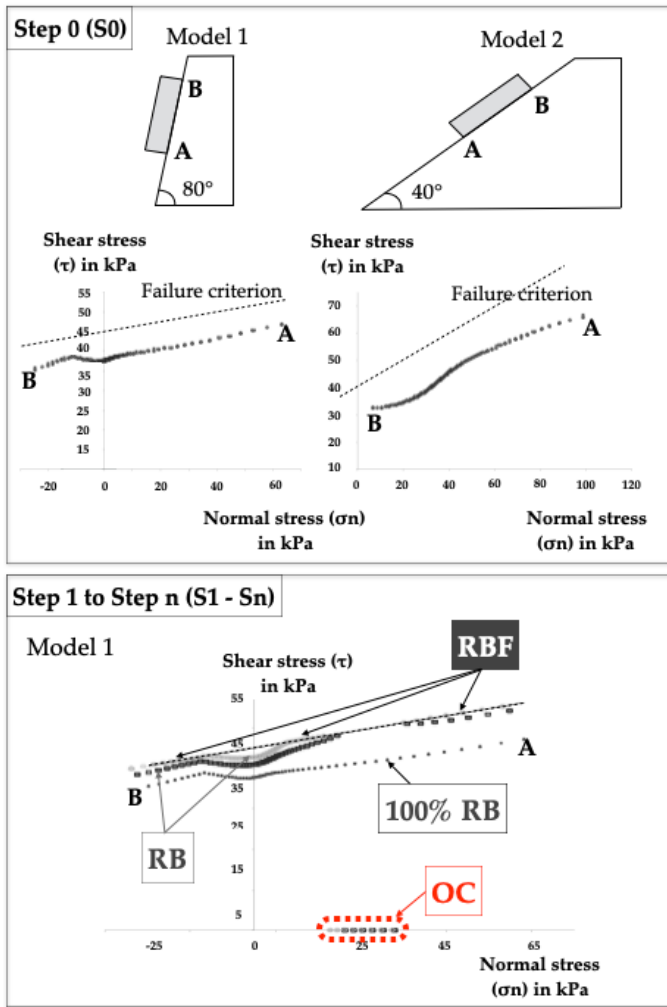
Fig. 3. Modelling process. Step 0: 100% of the rock joint is defined as Rock Bridge (RB). Step 1 to Step N: introduction of open crack (OC) along the joint. From Step 2 to Step n, it can be observed in the graph of the Model 1 the increase of shear stresses due to the introduction of OC.
