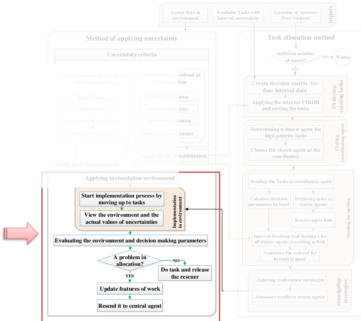
Figure 2 Task allocation flowchart in the proposed approach by five steps and environmental simulation
