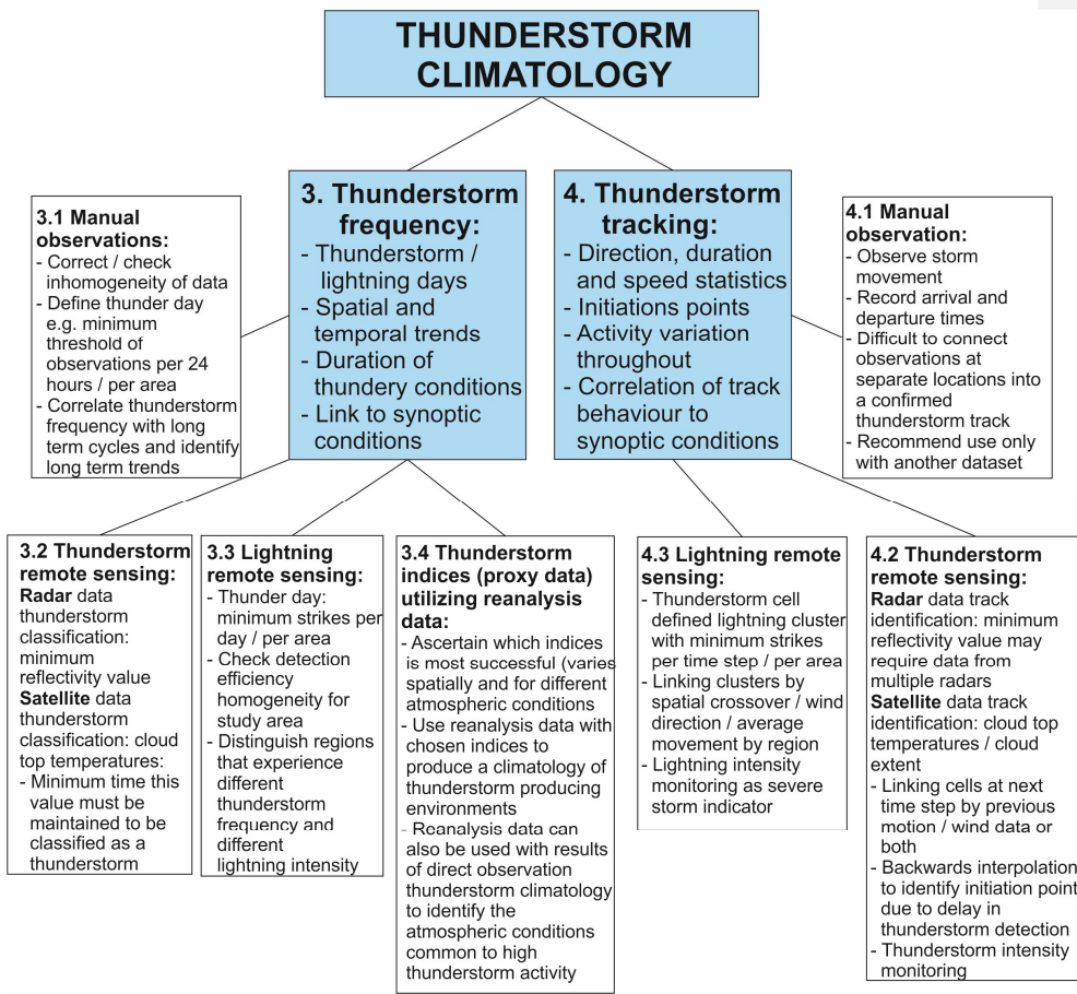
Figure 3: Diagrammatic summary of the potential research findings and data utilisation for a thunderstorm climatology created using either -thunderstorm frequency or thunderstorm tracking methodologies.
