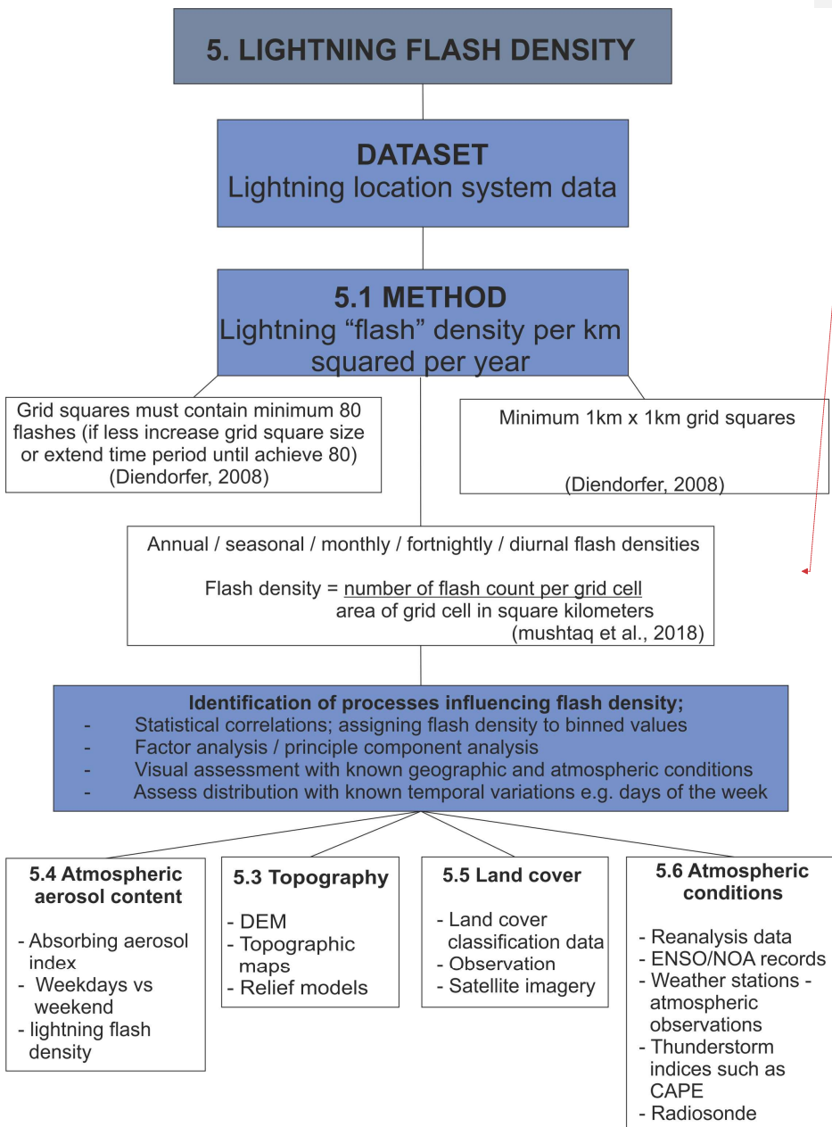
Figure 4: Diagrammatic summary of the steps involved in producing a lightning- flash density thunderstorm climatology, showing and the different variables to consider during the study design stage.
