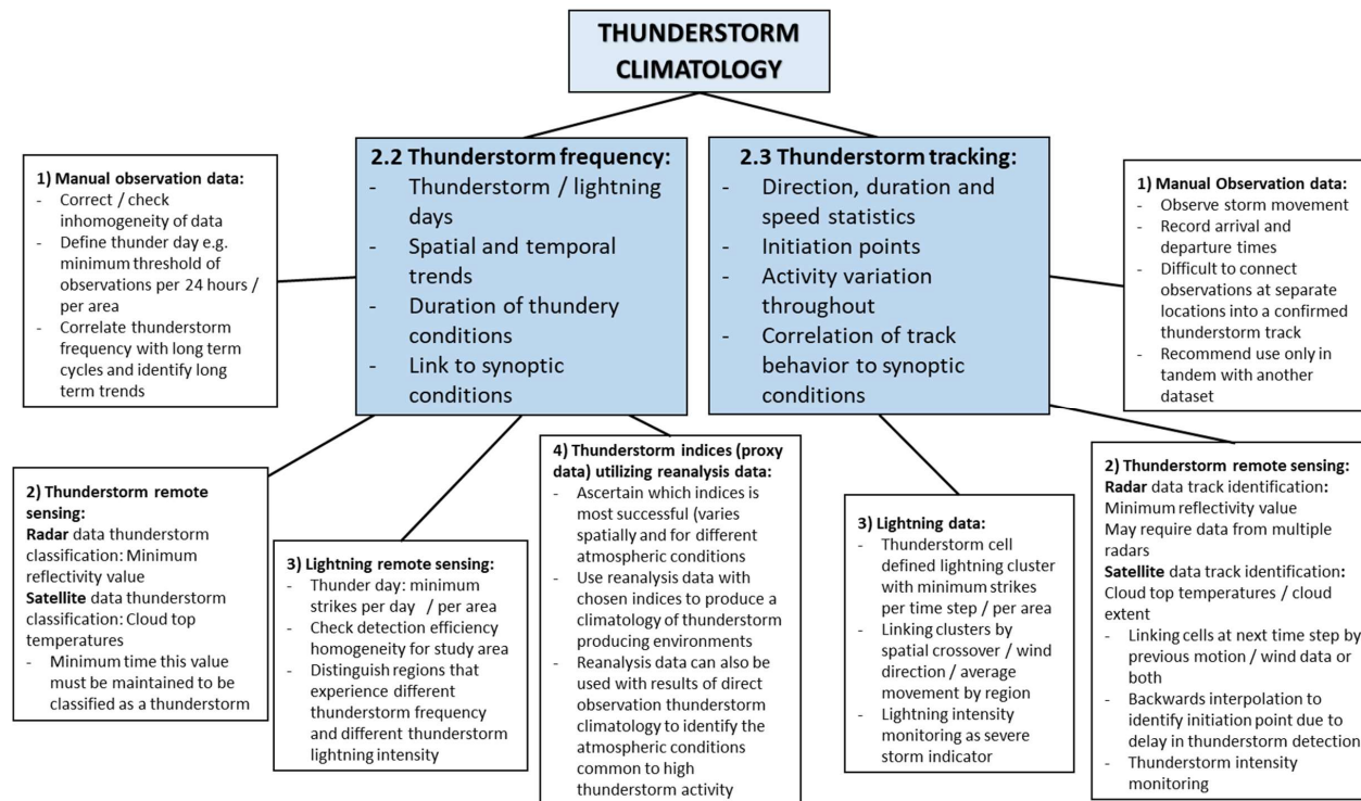
Figure 3: Diagrammatic summary of the potential research findings and data utilisation for a thunderstorm climatology created using either thunderstorm frequency or thunderstorm tracking methodologies.
