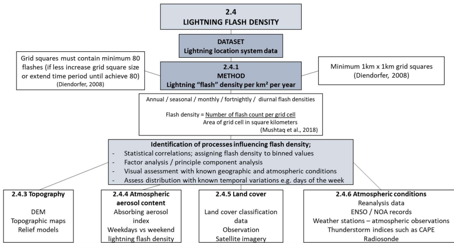
Figure 4: Diagrammatic summary of the steps involved in producing a lightning flash density thunderstorm climatology and the different variables to consider during the study design stage.
