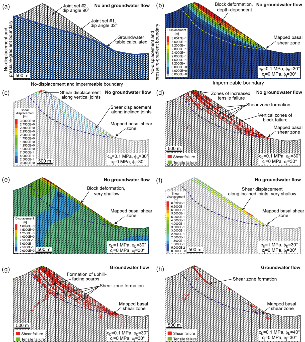
Figure 8. TS1 Results of modelling scenario I: (a) model set-up presenting the joint network and the calculated groundwater situation, (b) depth-dependent distribution of block displacements by implementing a block cohesion of c_b = 0.1 \text{ MPa} and internal friction angle of \phi_b = 30^\circ , (c) spatial distribution of shear displacements along joints ( c_b = 0.1 \text{ MPa} , \phi_b = 30^\circ ), (d) formation of multiple shear and antithetic zones due to block shear failure in a line-shaped arrangement ( c_b = 0.1 \text{ MPa} , \phi_b = 30^\circ ), (e) model run showing very shallow block displacements when block cohesion was increased from c_b = 0.1 to c_b = 1 \text{ MPa} ( \phi_b = 30^\circ ), (f) shallow-occurring shear displacements along joints for c_b = 0.1 \text{ MPa} TS2 and \phi_b = 30^\circ , (g) model run considering groundwater flow showing the formation of multiple shear and antithetic zones (i.e. uphill-facing scarps) due to block shear failure ( c_b = 0.1 \text{ MPa} , \phi_b = 30^\circ ), and (h) model run with groundwater flow showing the formation of a single shear zone being initiated mainly in the summit area and at the foot of the slope when the friction angle is increased to \phi_b = 40^\circ ( c_b = 0.1 \text{ MPa} ). All model runs presented reached stabilization.
