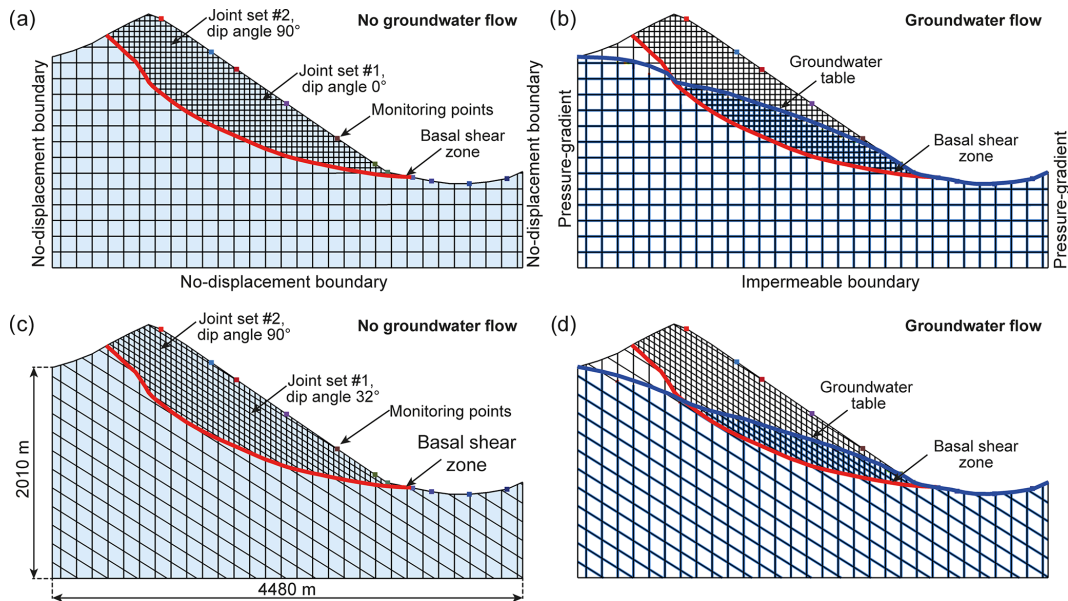
Figure 9. Model set-up and groundwater conditions of modelling scenario II: (a) model geometry characterized by a fully persistent horizontal (dip angle 90^\circ ) and vertical (dip angle 0^\circ ) joint set and the reconstructed basal shear zone (no groundwater flow), (b) same model geometry as in (a) but by considering groundwater flow, (c) model geometry characterized by a fully persistent inclined (dip angle 32^\circ ) and vertical joint (dip angle 0^\circ ) set and the reconstructed basal shear zone (no groundwater flow), and (d) same model geometry as in (c) but by considering groundwater flow. Monitoring points are included to prove if model runs have reached equilibrium (unbalanced forces) and stabilization (i.e. no ongoing displacements).
