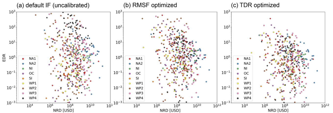
660 Figure A3: No significant correlation between event damage ratio (EDR) and normalized reported damage (NRD) was found. The scatter plots show the relationship for 473 TC events worldwide computed with three different sets of impact functions: (a) uncalibrated default ( V_{half}=74.7 \text{ ms}^{-1} ), (b) RMSF optimized, and (c) TDR optimized. The nine calibration regions are differentiated by color.
