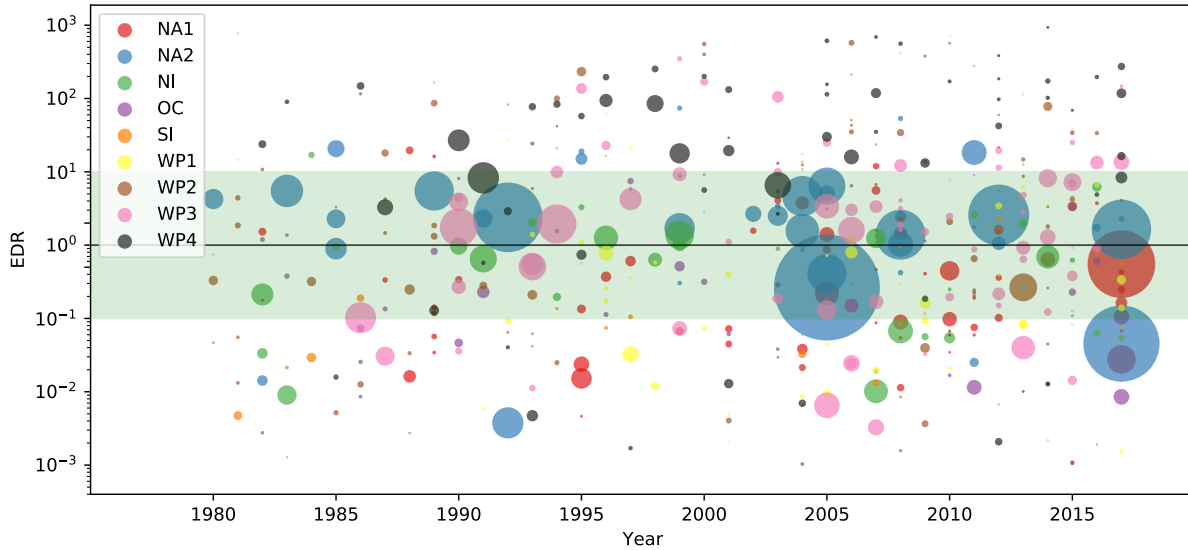
650 Figure A1: Event damage ratio (EDR) from 1980 to 2017 for matched 473 TC events worldwide. The nine calibration regions are differentiated by color. The area size of the dots represents the absolute normalized reported damage (NRD) per event. The green shading demarcates the range from EDR=0.1 to 10.
