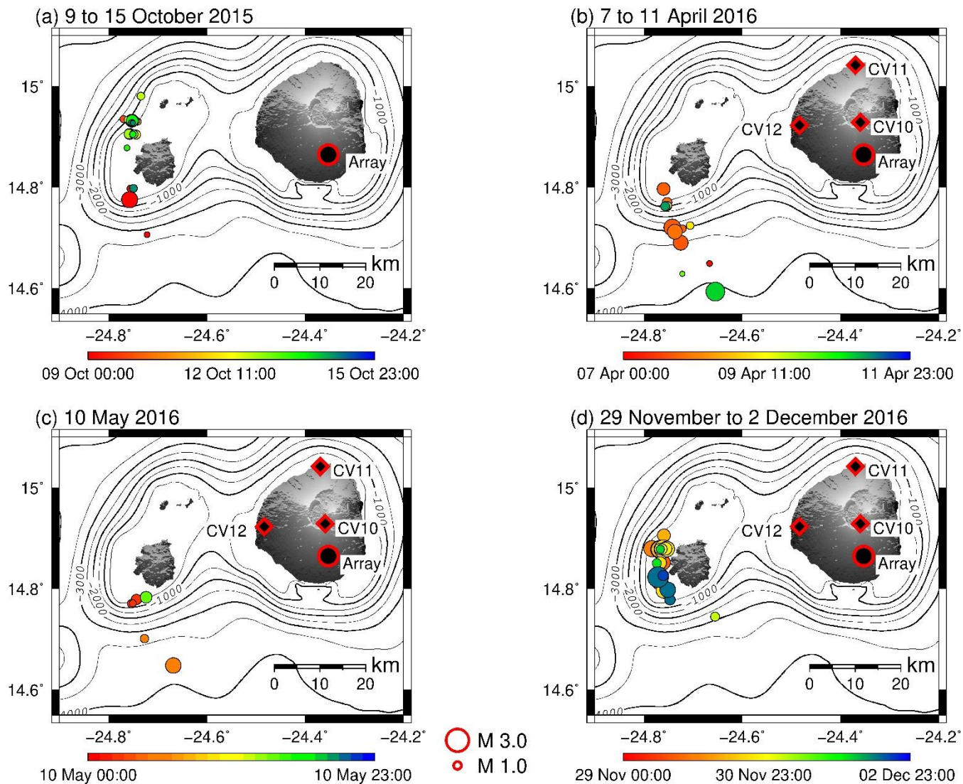
460 Figure 10: Earthquake locations for four different time periods of elevated seismicity. (a) 9–15 October 2015, (b) 7–11 April 2016, (c) 10 May 2016, (d) 29 November to 2 December 2016. Red/black circle: position of the array, red/black diamonds: additional broadband stations on Fogo. Topographic and bathymetry data are from Ryan et al. (2009).
