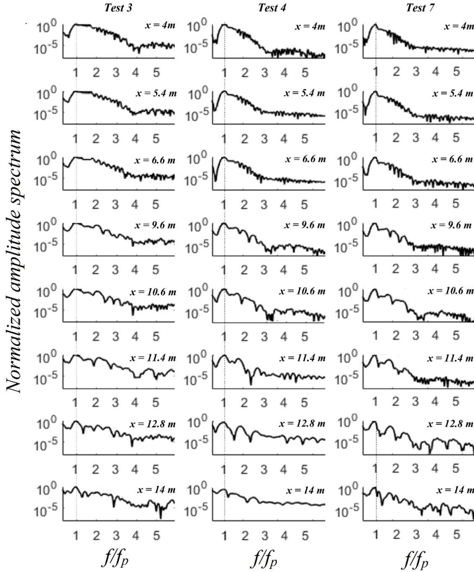
215 Figure 4 : Spatial evolution of normalised amplitude spectra in a log scale for Tests 3, 4 and 7.
