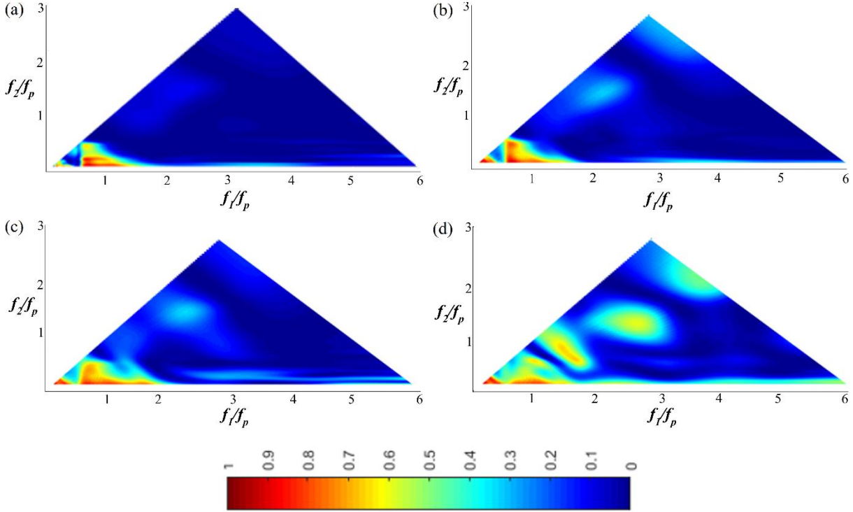
230 Figure 5 : The wavelet-based bicoherence spatial evolution on the flat bottom for a Pierson-Moskowitz wave train (Test 3). (a): x = 4 \text{ m} ; (b): x = 5 \text{ m} ; (c): x = 8 \text{ m} ; (d): x = 9.6 \text{ m} .
