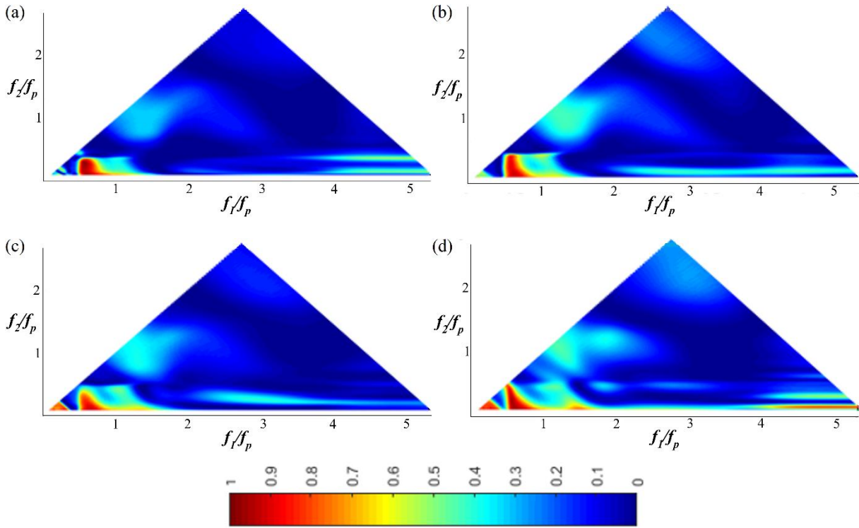
Figure 9: The wavelet-based bicoherence spatial evolution on the flat bottom for JONSWAP ( \gamma = 7 ) wave train (Test 7). (a): x = 4 m; (b): x = 6.4 m; (c): x = 8 m; (d): x = 9.6 m.
