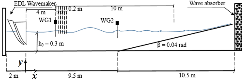
100 Figure 1: Schematic experimental setup, WG1 and WG2 denote wave gauge n°1 and wave gauge n°2 respectively.
