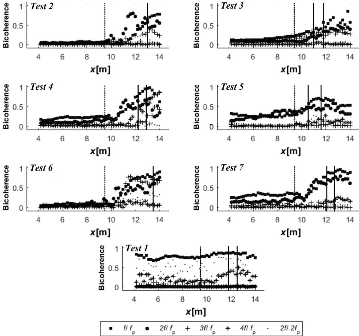
325 Figure 11: Spatial variation of the wavelet-based bicoherence among harmonics.
