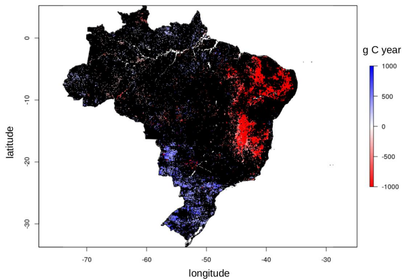
Fig. 7. Trends of primary productivity of vegetation based on the GOSIF dataset between 2009-2015. Areas in black showed non-significant.
