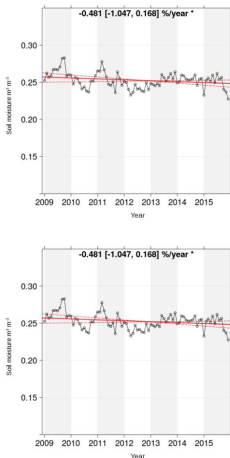
Figure 4: Brazil soil moisture trend from 2009 to 2015
