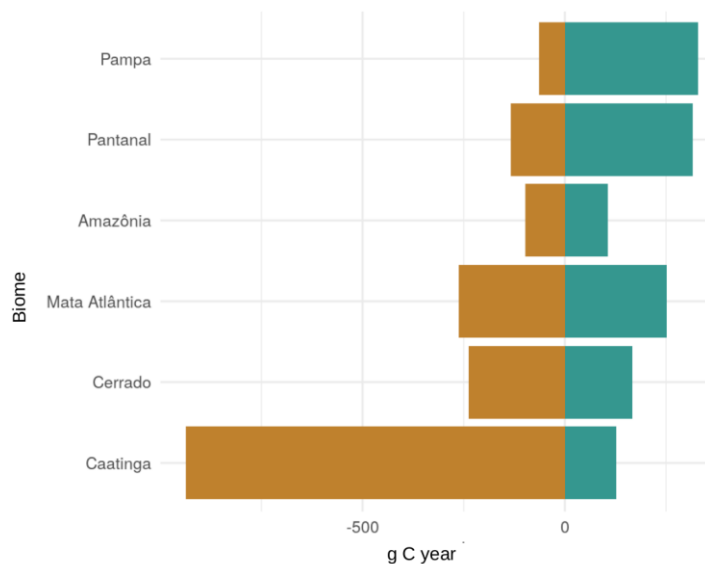
Fig. 8 Primary productivity trends across Brazilian biomes based in the GOSIF-GPP product across the analyzed period of time (2009-2015).
