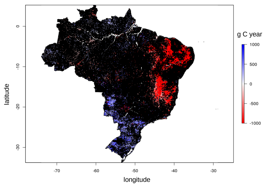
Fig. 1. OCO-2_GPP_BRazil_2009-2015
