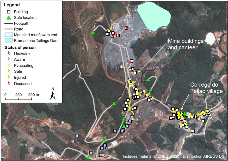
Figure 9: An example of an output from the LSM emergency planning modelling 90 seconds after the Brumadinho tailings dam failure assuming a warning is issued at the time of the breach The report number of fatalities as a result of the Brumadinho tailings dam failure was probably between ~270 and ~310 (Mining Journal, 2020; Keaveny, 2019). The results of the LSM model indicated that with no warning there would 456 fatalities out of the 502 people assumed to be at risk, a 91% fatality rate, with a warning at the exact time the dam failed there would have been 354 fatalities. Figure 10 shows the distribution of the fatalities and the status of the people at risk for the representation of the January 2019 disaster with no warning. The diameter of each circle in Figure 10 is in proportion to the number of people at each of the specific locations. The actual event is probably best represented by a combination of no warning scenario on
