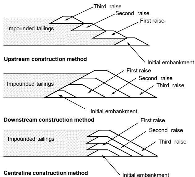
Figure 1: Different methods of construction for tailings dams
