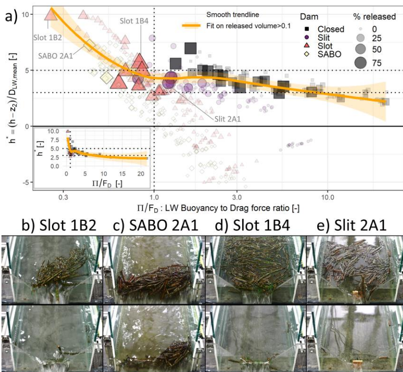
Figure 11: Characterizing release conditions: a) Dimensionless overtopping depth h^* VS buoyancy to drag force ratio \Pi/F_D with dot size and opacity proportional to the amount of LW released. Inset: same figure with non-logarithmic x-axis highlighting the sharp increase in h^* for significant releases; and (b-e) pictures of selected releases before (top picture) and after (bottom picture) releases. Releases occur for lower h^* in the \Pi/F_D \gg 1 domain, i.e., if buoyancy prevails and floating carpets forms with loosely packed logs (see d & e); while releases occur for higher h^* if dense jams forms under high drag forces in the \Pi/F_D < 1 domain where densely packed jams forms (b & c), eventually stabilized by protruding logs (see b, bottom picture)
