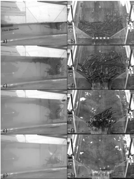
295 Figure 5 : Example of phases observed during runs where overtopping occurred (illustrated here with Mix A2, repetition #2 on slot dam) : Phase 1 – LW simply stuck at the dam, a few floating LW apart, here at discharge 0.5 L/s, (a) side view and (b) top view ; Phase 2 – slots jammed and floating carpet developed upstream, here at discharge 3.5 L/s, (c) side view and (d) top view ; Phase 2 later – denser jam for higher discharge (here at 5.4 L/s), several pieces yet released, (e) side view and (f) top view and, 5 second later the LW overtopped the barrier and Phase 3 – final state after jam overtopping occurs here still for discharge 5.4 L/s, (g) side view and (h) top view
