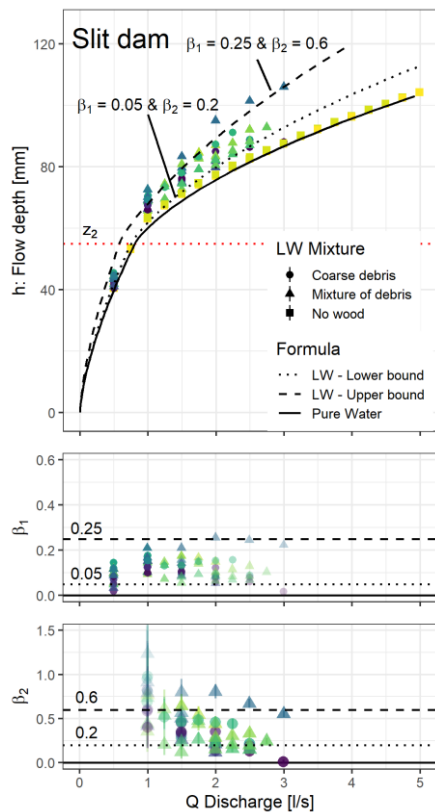
325 Figure 7. Flow depth versus discharge for gridded-slit dam and back-calculated \beta_1 and \beta_2 values, each color shade corresponds to a different run
