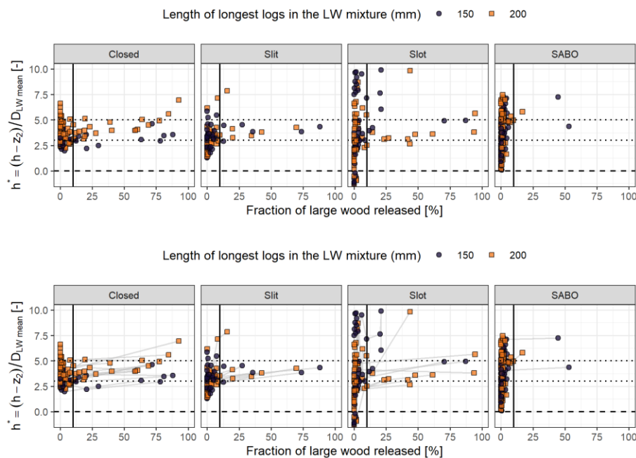
Figure 10. Percentage of LW released (i.e. mass fraction of LW released during one discharge step over total sample mass) against dimensionless overtopping depth h^* . Light grey lines connect points of each single runs. The continuous vertical line marked the 10% released that was fixed arbitrarily as the threshold value for significant LW release. Most significant LW release appear for 3 < h^* < 5 but discharge steps with absence of releases also appear often as illustrated by the numerous point on the left hand side of each graphs.
