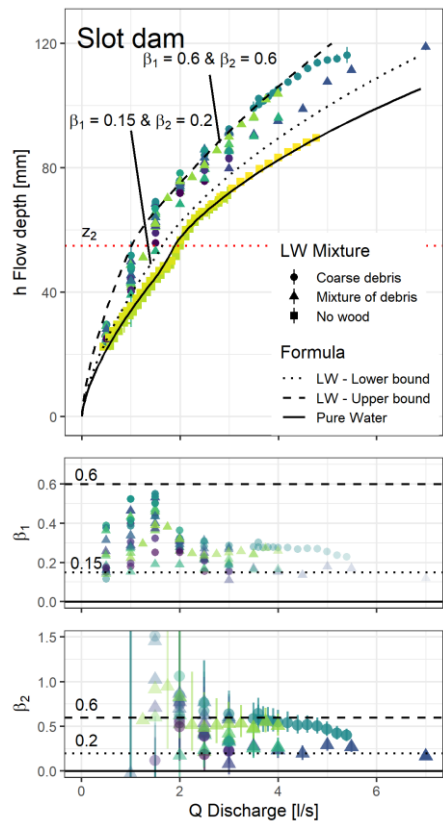
Figure 8. Flow depth versus discharge for slot dam and back-calculated \beta_1 and \beta_2 values, each color shade corresponds to a different run
