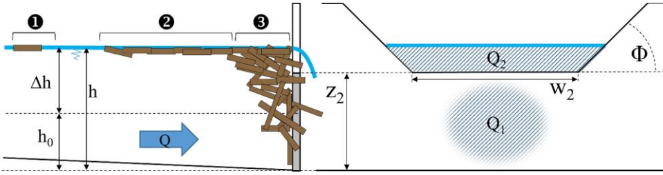
105 Figure 1. Notation used throughout the paper: a) side view of LW jamming a barrier and b) front view of barrier. Water depth without LW and with LW are denoted h_0 and h , respectively. The difference between h and h_0 is the head loss \Delta h . Dam crest is of height z_2 . Logs may be (1) freely flowing, (2) floating in a single layer as a carpet or (3) jamming the barrier with most pieces submerged. The total water discharge Q is split into Q_1 , the discharge passing through the dam and Q_2 the discharge overflowing the dam.
