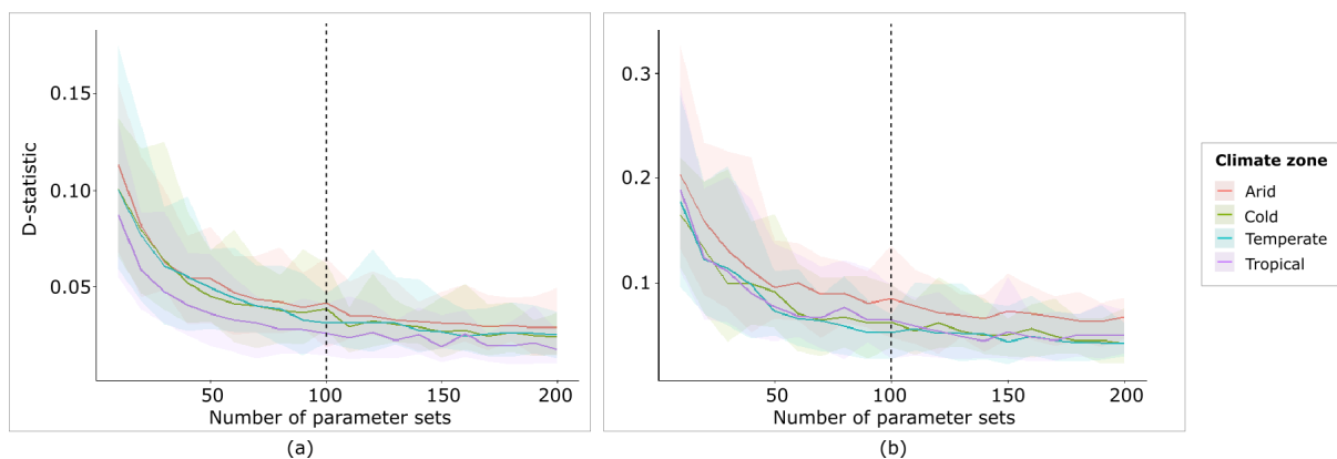
Figure 2. D-statistics for maximum (a) and minimum runoff (b) in one model structure (UL1) with twelve parameters, which result from the Kolmogorov-Smirnov test. The other model structures show a similar trend (not shown). The bands are a result of the different parameter samples, the different colours represent the four climate zones.
