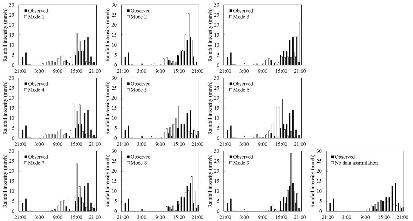
Figure 8. Time series bars of observed and simulated areal rainfall with nine data assimilation modes and the rainfall observation for Event II.
