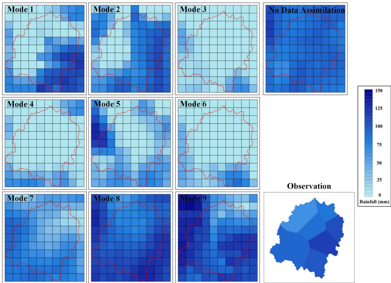
Figure 4. Spatial distribution of the simulated 24 h rainfall accumulations with nine data assimilation modes for Event I.
