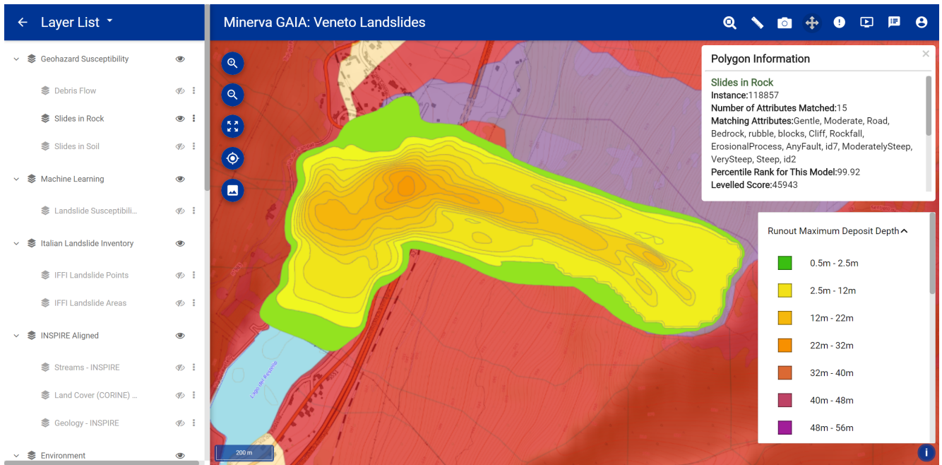
Figure 7. Landslide runout and Screen capture of the web map showing layer list, information popup in Web Map window, map legend, and landslide runout. Base map credit: © OpenTopoMap (CC-BY-SA)
