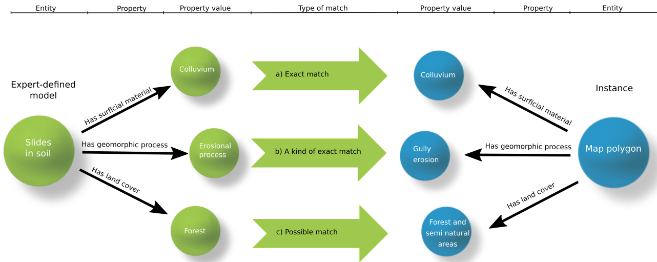
Figure 2. Graphical representation of the matching process between expert-defined models and map polygon instances. a) is an example of an Exact exact match between the property value “ Colluvium colluvium”; b) is an example of a kind of (AKO) exact match, because “gully erosion” is a more specific kind of “erosional process”. The model is looking for an “erosional process” and found a “gully erosion”; c) is an example of a possible exact match because “ Forest forest and semi natural areas” is a broader concept of “ Forest forest”. The model is looking for “forest” but we do not know whether the instance is a “forest”. We only know that the instance is “forest and semi natural areas”. The vocabulary and the hierarchy are controlled by the ontology. Note that frequency terms for model properties are not shown in this figure.
