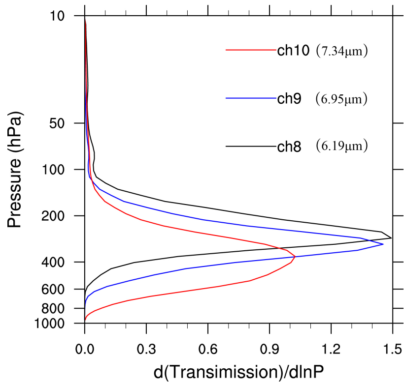
Fig. 1. Fig.1 Weighting function for Channel 8, 9, and 10.
