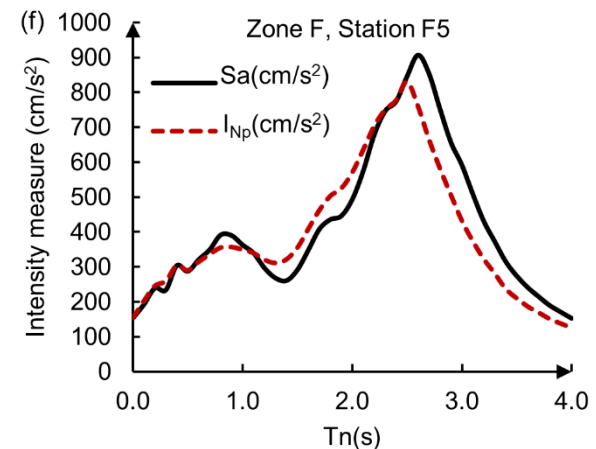
735 Figure 7: Uniform hazard spectra of S_a(T_1) and I_{Np} , corresponding to one representative station of each zone listed in Table 1, considering 250 year-return interval.
