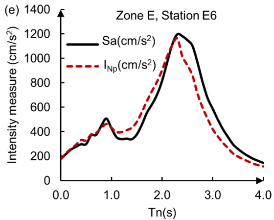
735 Figure 7: Uniform hazard spectra of S_a(T_1) and I_{Np} , corresponding to one representative station of each zone listed in Table 1, considering 250 year-return interval.
