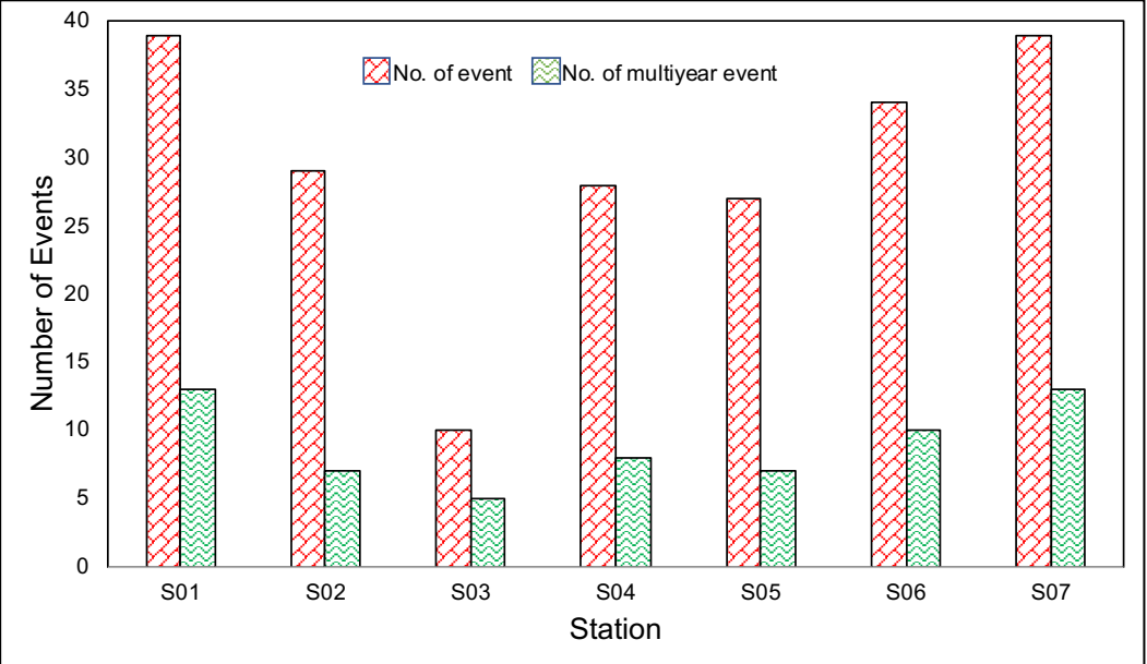
785 Figure 7: Number of drought events.
