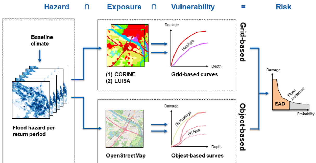
135 Figure 1 Graphical representation of the risk assessment using the grid-based approach (top-row) with the (1) CORINE and (2) LUISA land cover grids and the object-based approach (bottom-row) with OpenStreetMap and (3) the Huizinga and (4) a set of new damage curves © OpenStreetMap contributors 2019. Distributed under a Creative Commons BY-SA License
