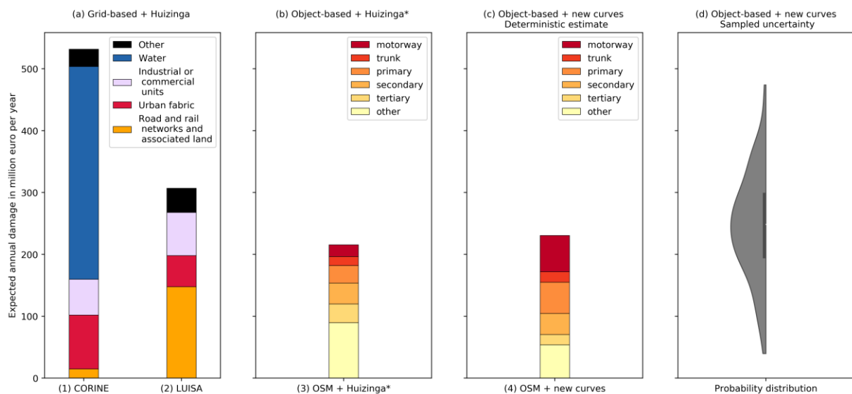
Figure 5 Flood risk of the European road network according to the grid-based and the object-based approach (a) Grid-based approach with (1) CORINE and (2) LUISA + the Huizinga damage curves, per land cover type (b) Object-based approach + *object translation of Huizinga damage curves (3), per road type
