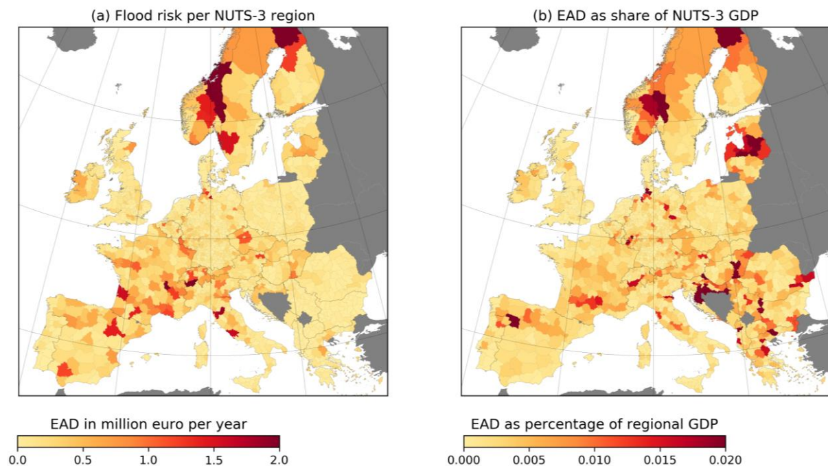
Figure 5 Expected annual damage (EAD) to road infrastructure aggregated by NUTS-3 region. The left-hand panel presents the absolute values, the right-hand panel expresses the EAD as percentage of the GDP per NUTS-3 region.
