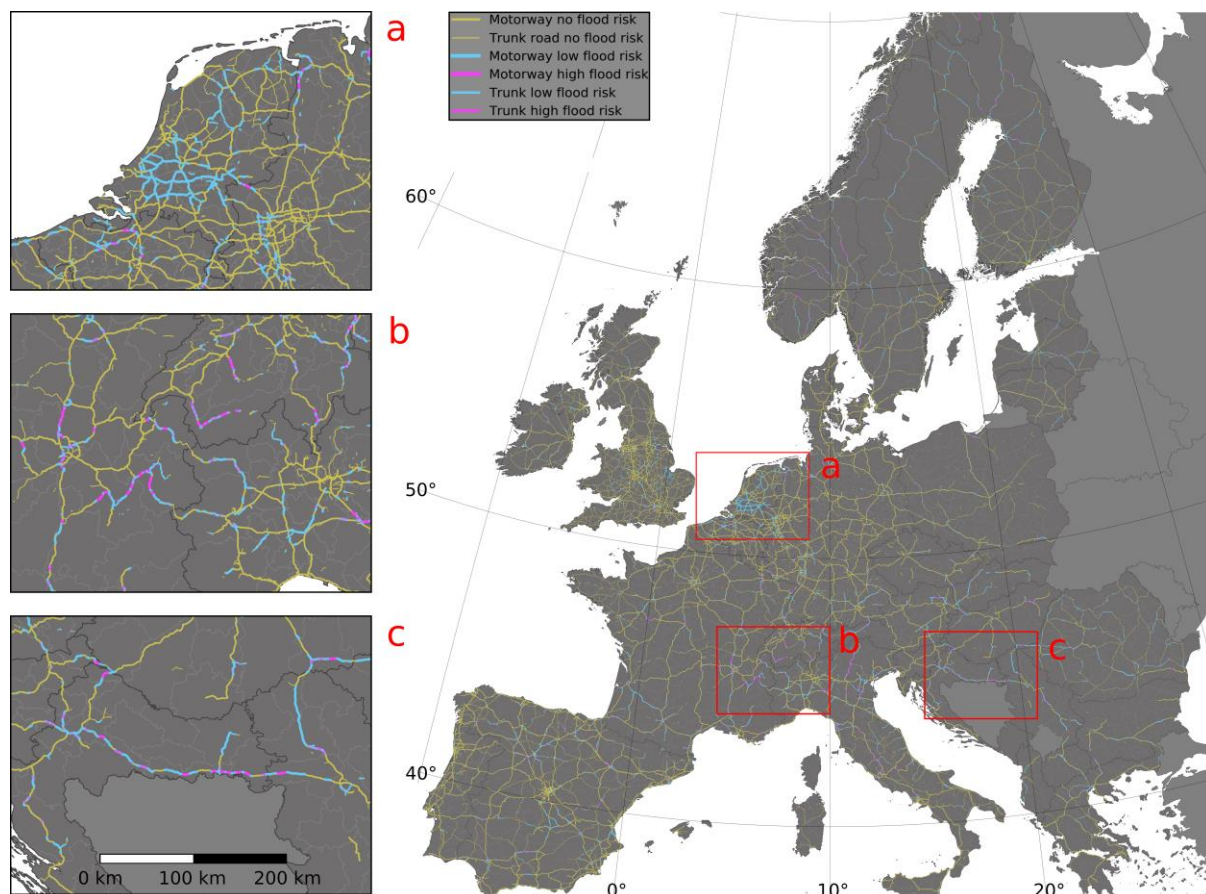
Figure 6 Flood risk of motorways and trunk roads in the European main road network, see Figure S9 for a high-resolution version. Road geometries © OpenStreetMap contributors 2019. Distributed under a Creative Commons BY-SA License.
