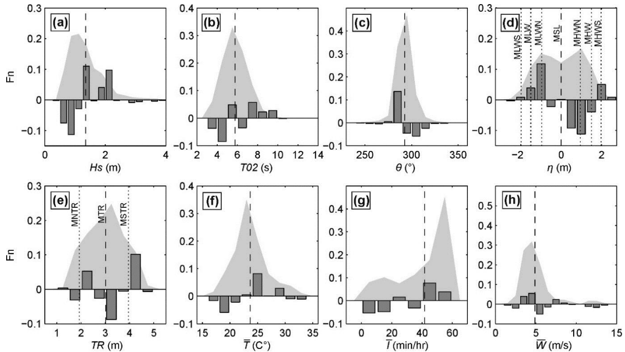
Figure 5: Environmental controls on rip related SZIs: normalised frequency distributions F_n during the summers of 2007, 2009 and 2015 (light grey region), referred to as ‘average’ background distribution, of (a) significant wave height H_s ; (b) mean wave period T_{02} ; (c) wave direction \theta ; (d) water level \eta ; (e) daily tide range TR ; (f) daily-mean air temperature \bar{T} ; (g) daily-mean hourly insolation \bar{I} and (h) daily-mean wind speed \bar{W} , with in all panels the dark grey bars showing the difference between the surfing related and the ‘average’ background distributions and the vertical dashed line showing the background mean.
