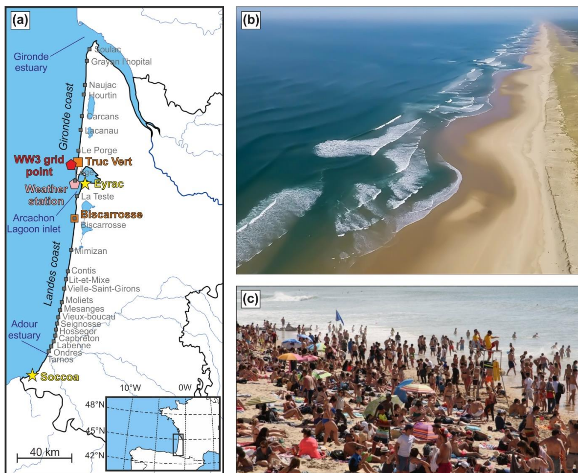
Figure 1: (a) Location map of SW France showing the 230 km long sandy beach study location encompassing the Gironde and Landes between the Adour and Gironde estuaries. Grey squares indicate coastal municipalities where incident/injury report forms were gathered, yellow stars indicate tide gauges, and the red and pink polygons show the location of the WW3 model output grid point and weather station, respectively. (b) Aerial photograph of Truc Vert beach taken at low tide showing a landscape representative of the SW France beaches with deep rip channels and steeper upper beach slopes (Ph. V. Marieu). (c) Crowded beach during summer at high tide with lifeguards supervising a bathing area delimited by 2 blue flags, typically extending no more than 100 m alongshore (Ph. J. Lestage).
