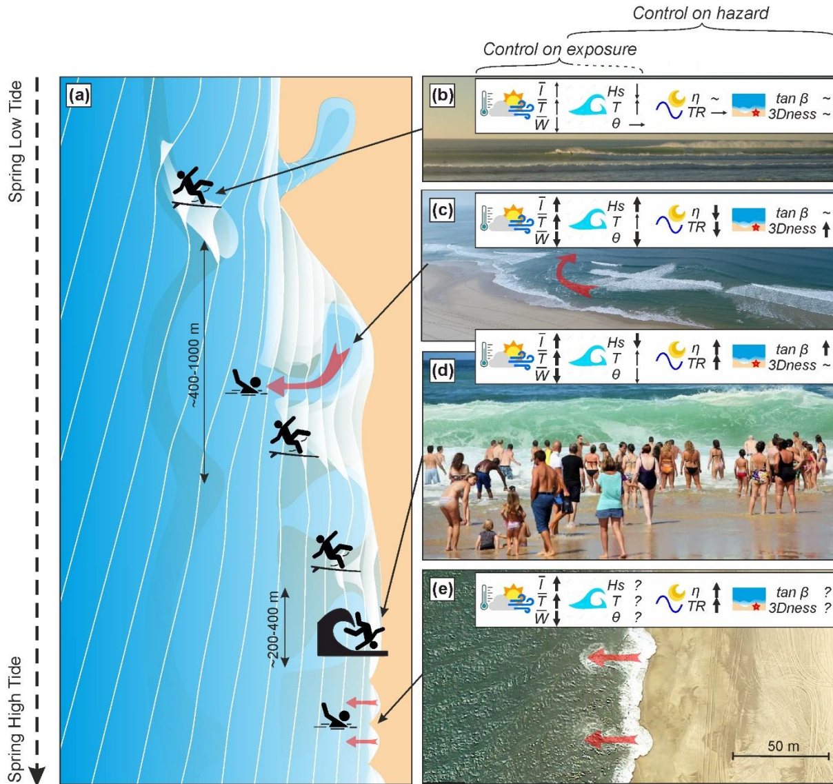
Figure 17: (a) Primary surf zone life risks along the sandy surf beaches of SW France with with: (b) high-risk surfing activity throughout the tide cycle; (c) channel rips primarily flowing between low tide and mid tide and maximized for near shore-normally long period swell; (d) hazardous shore-break waves primarily occurring at high tide on the steepest section of the beach and (e) small-scale swash rips flowing through the centre of beach cusps at spring high tide. The primary environmental controls on beachgoer exposure and surf-zone hazard are synthesised in the top boxes in panel (b-e), with bold arrows, '~' and '?' indicating strong, absent and unknown control, respectively. Wave and morphological controls on swash rip life risk was not addressed here as it was not possible to discriminate from channel rips.
