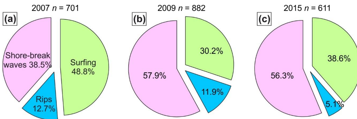
Figure 14: Percentage of SZIs by year : (a) 2007; (b) 2009; (c) 2015.
