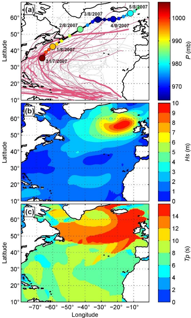
Figure 9: Atmospheric conditions and resulting wave fields causing the most hazardous rip conditions of the dataset along the SW France beaches on August 5 2007: (a) Trajectory, daily position (large circles) and minimum central pressure of tropical cyclone Chantal superimposed onto all tropical cyclone trajectories over the period 2007-2017 (light grey) and limited to the July-August summer periods (dark pink) and only summers 2007, 2009 and 2015 (thick dark pink); (b) Significant wave height H_s and (c) peak wave period field on August 4, 2h00 local time.
