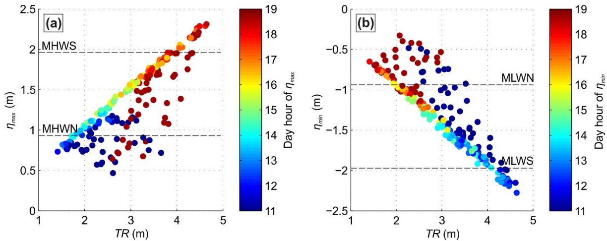
Figure 12: (a) Daily maximum tide elevation \eta_{max} during lifeguard patrolled hours versus daily tide range TR with colour bar indicating the day hour of \eta_{max} occurrence; (b) daily minimum tide elevation \eta_{min} during lifeguard patrolled hours versus daily tide range TR with colour bar indicating the day hour of \eta_{min} occurrence.
