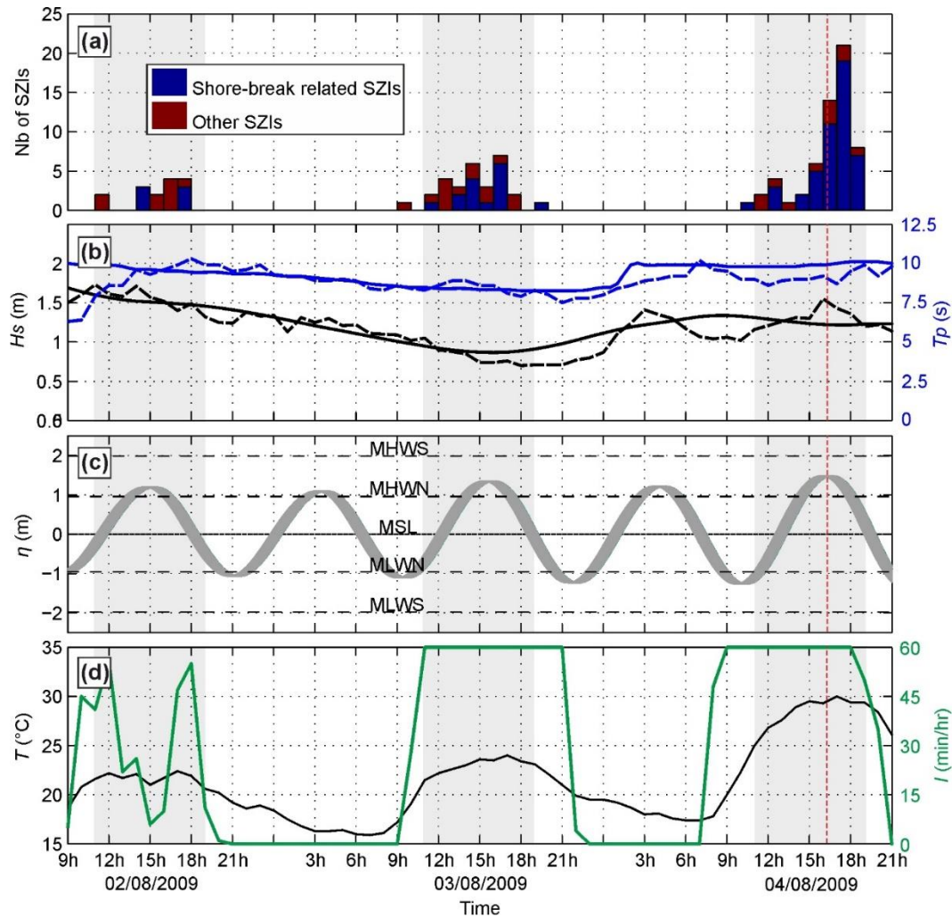
Figure 10: Time series on August 2-4 2009, with August 4 having the largest number of shore-break related injuries in the entire dataset, showing: (a) distribution SZIs with indication of shore-break related injuries; (b) significant wave height H_s and peak wave period T_p from the model (solid) and from the Candhis directional wave buoy in 50-m depth facing Truc Vert which only worked intermittently during the three summer seasons; (c) tide elevation \eta ; (d) hourly air temperature T and insolation I . In all panels, the light grey areas show lifeguard patrolled hours. In all panels, the vertical red dashed line indicates low tide occurrence on August 4 2009.
