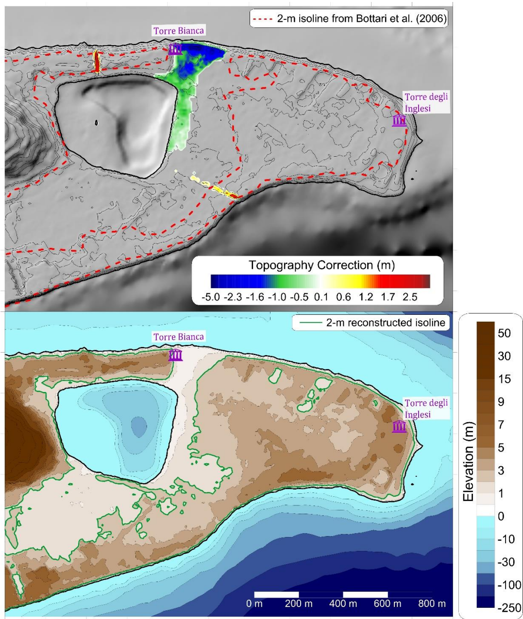
Figure 9. Upper panel: Shaded-relief map of the current topography of Capo Peloro, with 2-m isoline (red-dashed line) obtained from Bottari et al. (2006) showing the most likely connection between the lake and the sea, just east of Torre Bianca. The corrections are shown in green-blue when negative (meaning “digging” with respect to the present ground level) and in yellow-red when positive, meaning increased ground elevation. Lower panel: Contour plot of Grid 4, with the low topography from the north-eastern corner of the lake to the sea. In green, the new 2-m isoline is evidenced. With the corrected topo-bathymetry we have built the Grid 4 that has the same areal coverage as Grid 3.
