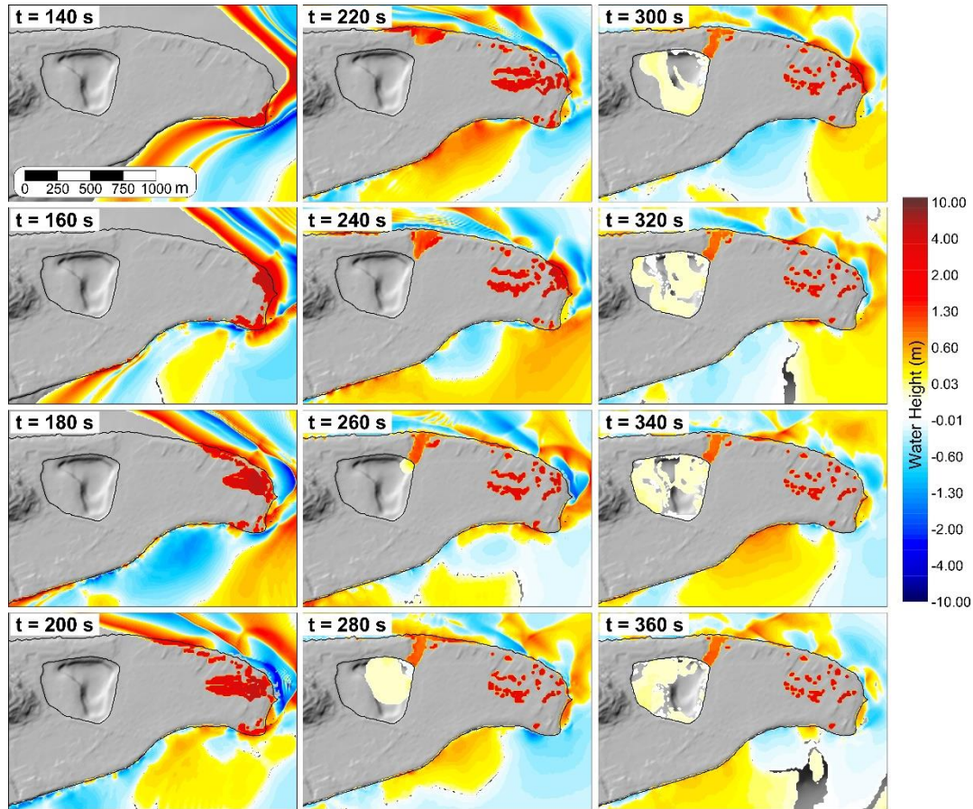
Figure 10. Propagation frames of the 1783 landslide-generated tsunami on the western part of Grid 4. Notice the water propagation inside the lake.
