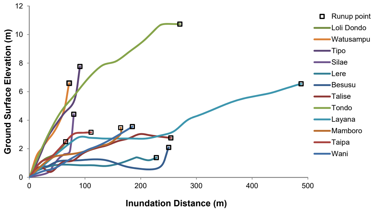
Figure 5: Transects of beach where tsunami wave arrived. The longest inundation distance is at the Layana site and the highest runup is at the Tondo site.
