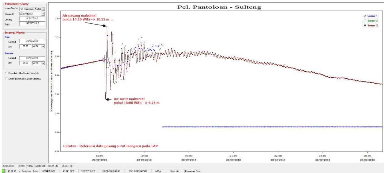
Figure 8: Water level recording at the Pantoloan tidal station managed by the Geospatial Information Agency (Sudibyo, 2018).
