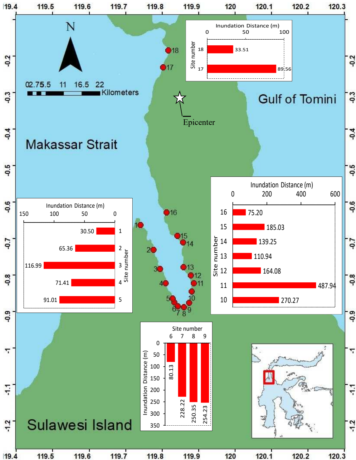
Figure 3: Measurement results of inundation distances.
