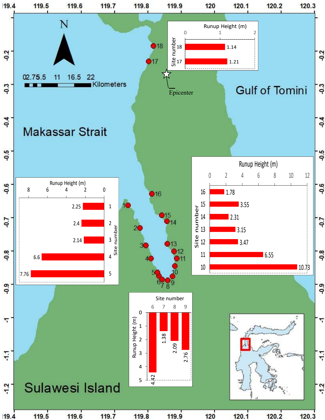
Figure 4: Measurement results of runup heights.
