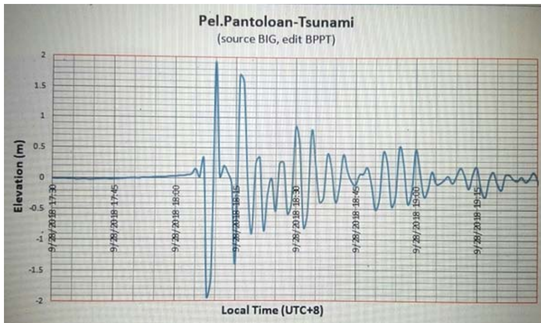
Figure 9: Magnified view of Fig. 8, sourced from the Geospatial Information Agency (Sudibyo, 2018).
