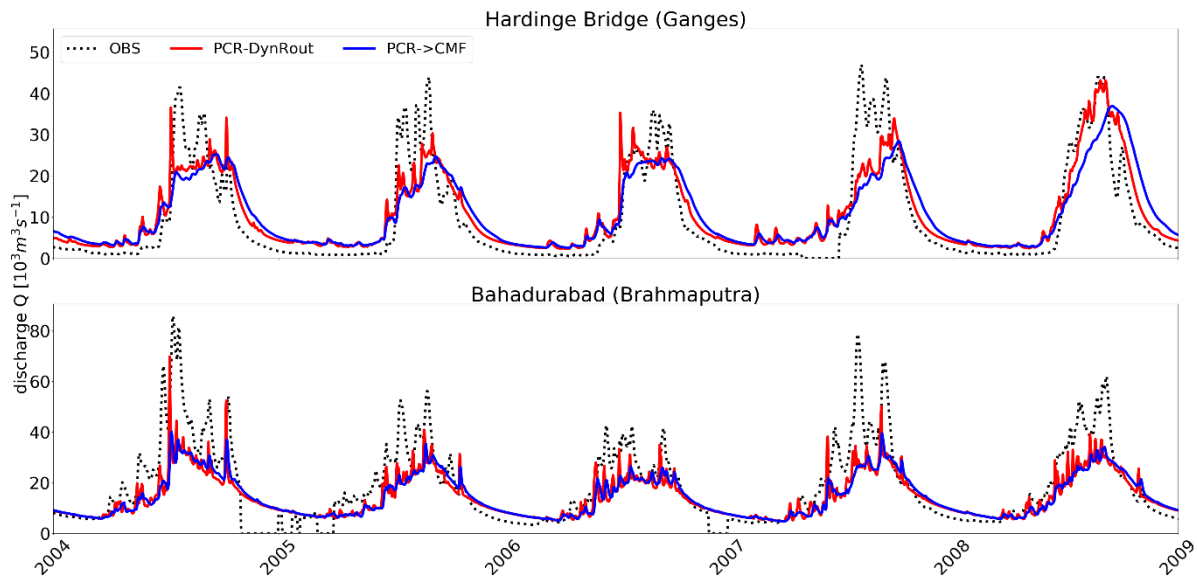
Figure 5: Simulated discharge by PCR-DynRout and PCR->CMF as well as observed discharge at both Hardinge Bridge (Ganges) and Bahadurabad (Brahmaputra)
