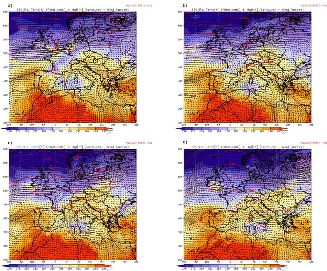
10 Fig. S1: (a-d) Temperature (filled-contours), geopotential height (red-contours) and wind vectors at 850-hPa every 12 h from 12 UTC on 19 august 2018 to 00 UTC on 21 august 2018. Maps from NCEP GDAS/FNL (0.25° resolution).
