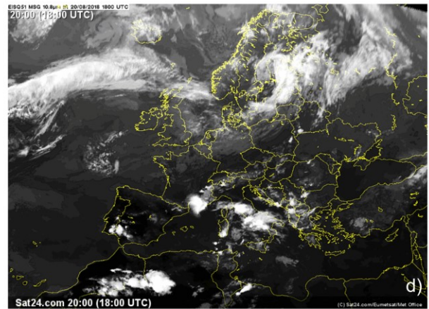
5 Fig. S2: (a-d) Satellite images of the thermal infrared channel ( 10.8 \mu\text{m} ) every 6 h from 00 UTC to 18 UTC on 20 August 2018. Source: www.sat24.com ; ©Eumetsat.
