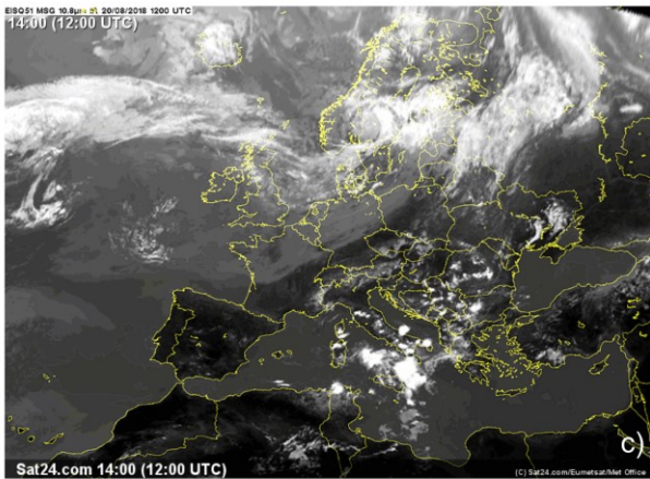
5 Fig. S2: (a-d) Satellite images of the thermal infrared channel ( 10.8 \mu\text{m} ) every 6 h from 00 UTC to 18 UTC on 20 August 2018. Source: www.sat24.com ; ©Eumetsat.
