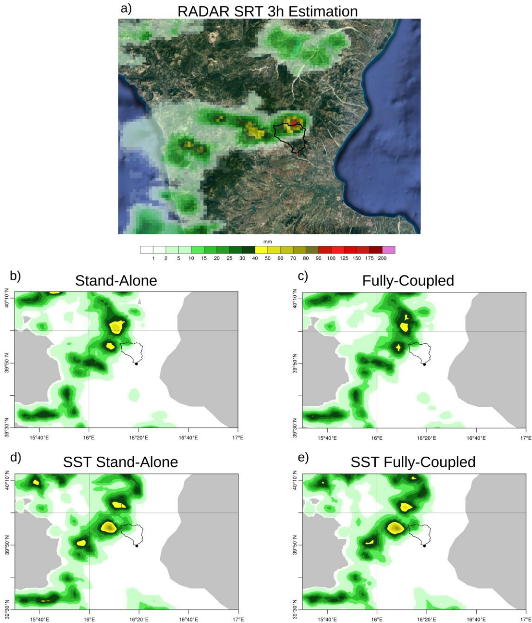
5 Fig. 2: a) 3h (10-13 UTC) Surface Rainfall Total (SRT) product derived by radar, provided by ‘The Regional Agency for the Protection of the Environment of Calabria region’ (source: http://www.cfd.calabria.it/DatiVari/Pubblicazioni/rapporto%20evento%202020%20agosto%202018.pdf , last access 1 March 2019); b) 3h (10-13 UTC) accumulated precipitation simulated by WRF for the run RUN_SA; c) as in b) for the run RUN_FC; d) as in b) for the run RUN_SST_SA; e) as in b) for the run RUN_SST_FC. The same colour-bar is used for all the maps. In Figs. from b) to e) the disaster site is identified by a black dot.
