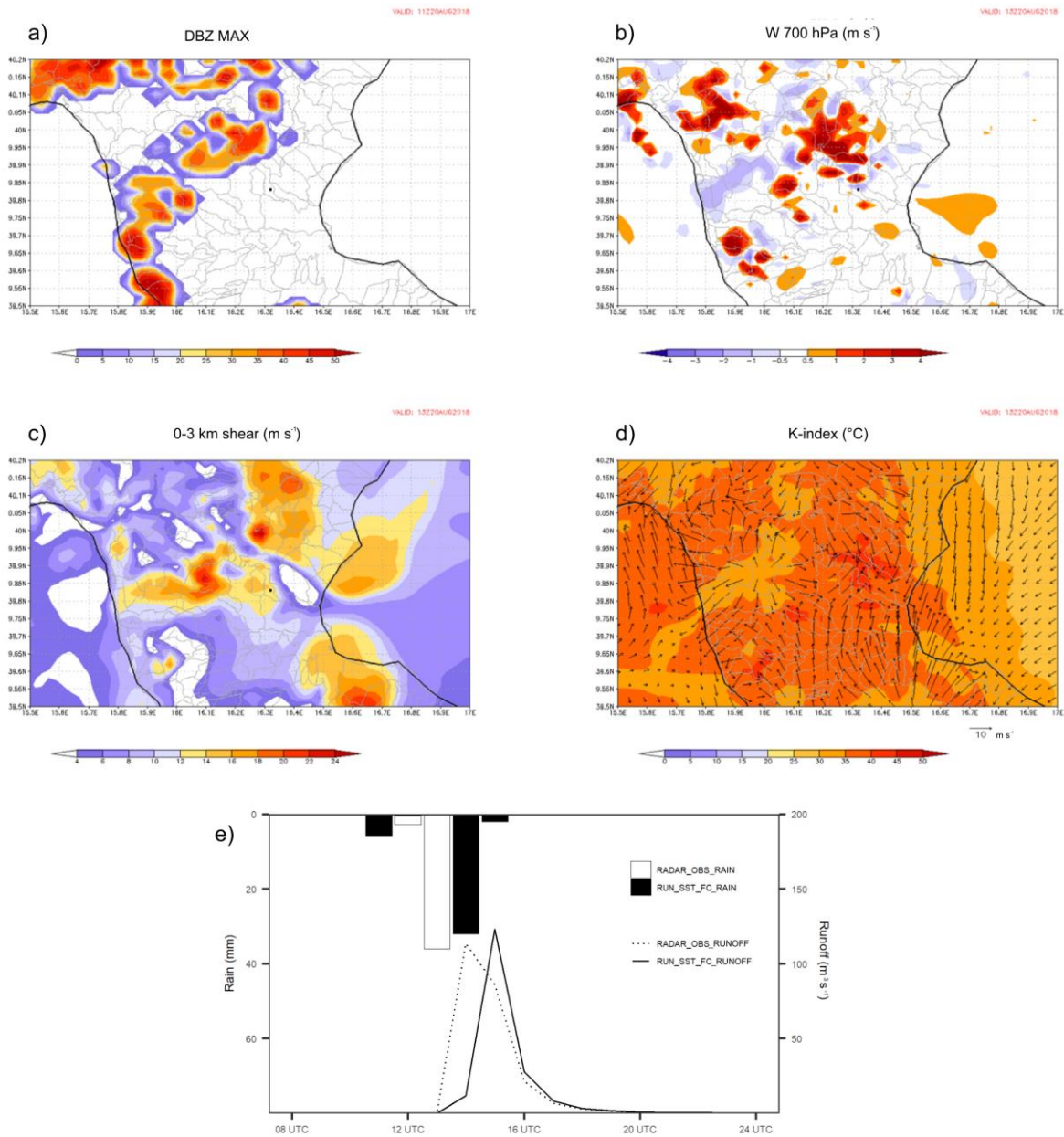
Fig. 3: a) maximum reflectivity simulated at 11 UTC (dBZ); b) 700 hPa vertical wind speed simulated at 13 UTC ( m s^{-1} ); c) 0-3 km wind shear simulated at 13 UTC ( m s^{-1} ); d) k-index simulated at 13 UTC ( ^{\circ}C ); e) hourly averaged rainfall values over the catchment (mm) and the resulting hydrograph ( m^3 s^{-1} ) achieved for radar-driven simulations and RUN_SST_FC. Results shown in
