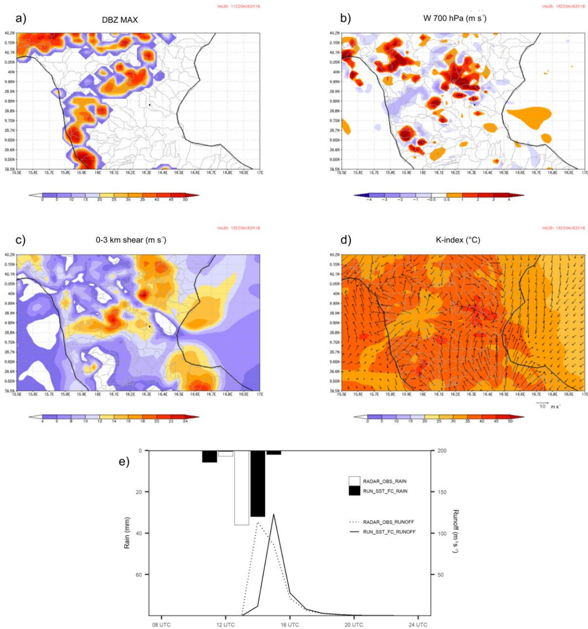
Fig. 3: a) maximum reflectivity simulated at 11 UTC (dBZ); b) 700 hPa vertical wind speed simulated at 13 UTC ( \text{m s}^{-1} ); c) 0-3 km wind shear simulated at 13 UTC ( \text{m s}^{-1} ); d) k-index simulated at 13 UTC ( ^{\circ}\text{C} ); e) hourly averaged rainfall values over the catchment (mm) and the resulting hydrograph ( \text{m}^3 \text{s}^{-1} ) achieved for radar-driven simulations and RUN_SST_FC. Results shown in
