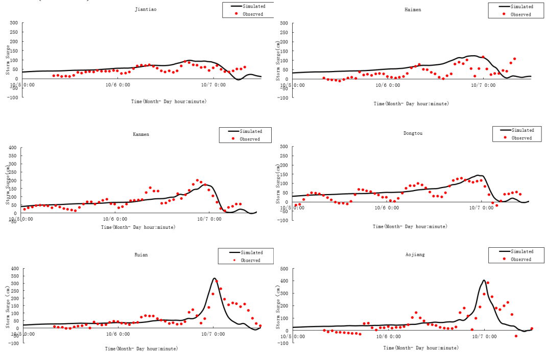
Fig. 6 Verification of the storm surge for tidal stations affected by the storm surge caused by Typhoon Fitow (No. 1323)
