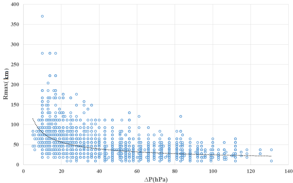
290 Fig. 10 The relation between the central pressure difference ( \Delta P ) and the radius of maximum wind ( R_{max} )
