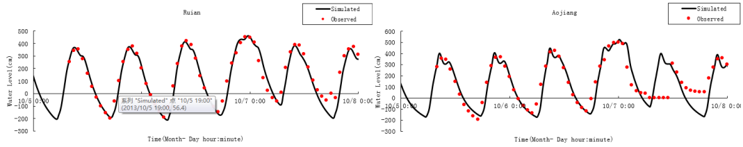
Fig. 5 Verification of the high tide level for tidal stations affected by the storm surge caused by Typhoon Fitow (No. 1323)
