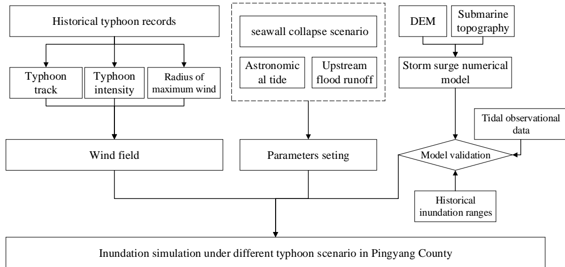
125 Fig. 2 Framework of storm surge inundation simulation under different typhoon scenario in Pingyang County
