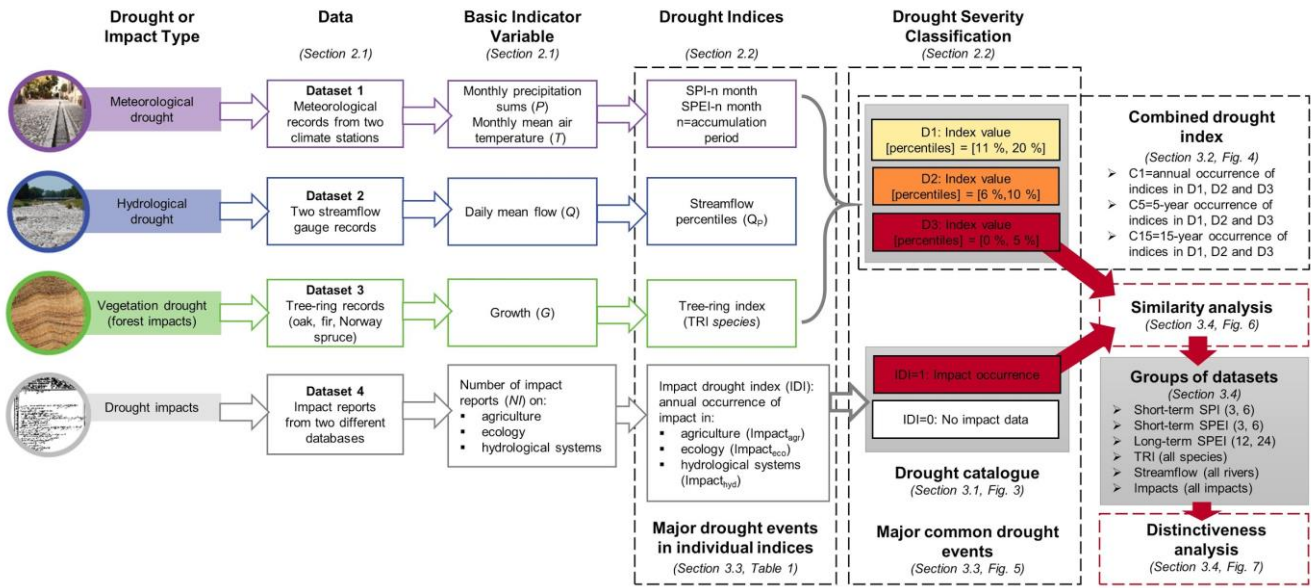
95 Figure 1: Conceptual overview of the multi-perspective approach of this study. The used multi-variable dataset is shown as well as the derived indices used to create the drought catalogue.
