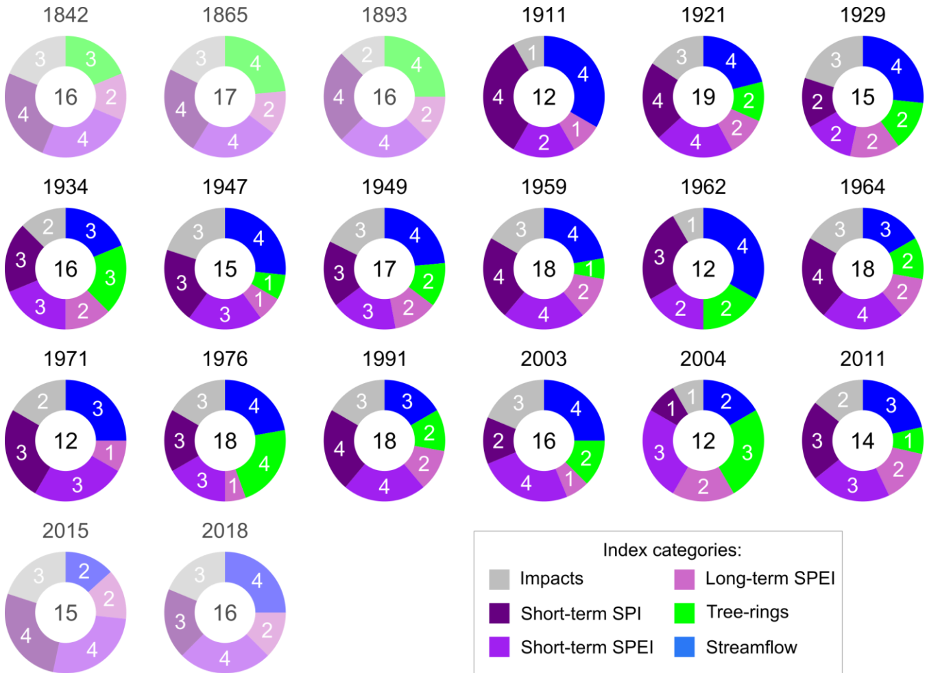
Figure 5: Drought years in which more than ten indices (from different categories) indicate a drought (the total number of indices pointing to a drought is written in the circle, the number of indices per group pointing to a drought is written in each section of the ring). Years without streamflow data (prior to 1900) or without tree-ring data (after 2011) are displayed with paler colors.
