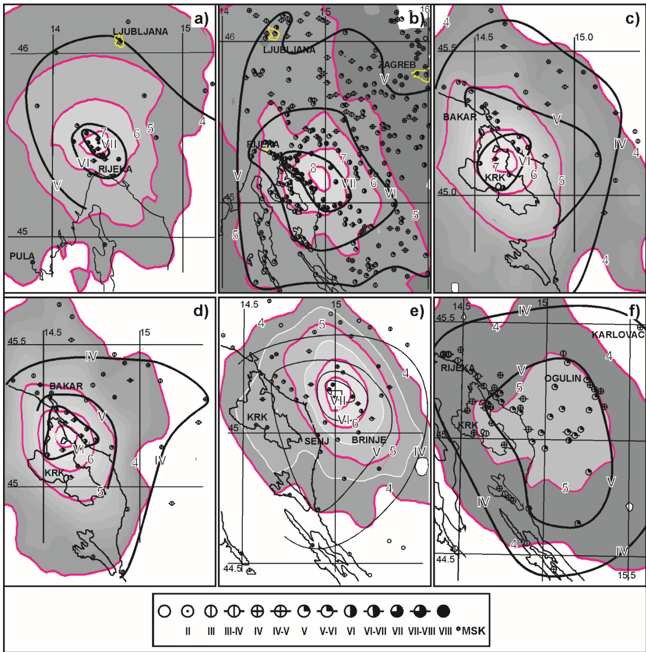
Figure 8: Empirical (black lines) and modelled (purple lines) isoseismal maps for the earthquakes occurred on: (a) 1 March 1870 at 19:57 UTC; (b) 12 March 1913 at 03:23 UTC; (c) 5 February 1939 at 22:00 UTC; (d) 6 February 5 1939 at 07:23 UTC; (e) 5 February 2007 at 08:30 UTC; 30 July 2013 at 12:58 UTC.
