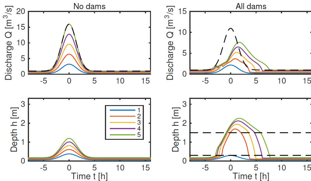
20 Figure 5: Solutions for a one-dimensional 5-node network as in figure 2b, forced by uniform inflow to each node q(t) = q_0 + q_{max} \exp(-t^2/\sigma^2) , with q_0 = 0.22 \text{ m}^3\text{s}^{-1} , q_{max} = 3 \text{ m}^3\text{s}^{-1} , and \sigma = 2 \text{ h} . Parameter values are as given in section 2.3, together with \lambda = 50 , b = 0.3 \text{ m} and H = 1.5 \text{ m} . Left-hand panels show the response with no dams, when the peak discharge is almost identical to the peak cumulative inflow, shown by the dashed line in the upper panels. Right-hand panels show the response if a dam is included on each of the 5 reaches. The dashed lines in the lower panel shows the heights of the bottom and top of the dams.
