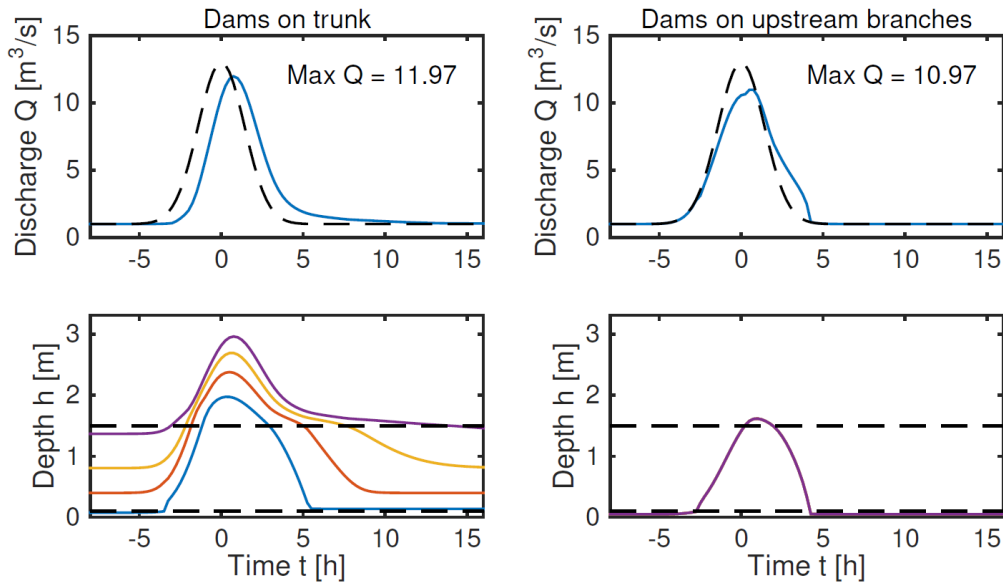
Figure 7: Solutions for a one-dimensional 5-node network as in figure 2b, forced by uniform inflow to each node q(t) = q_0 + q_{\max} \exp(-t^2/\sigma^2) , with q_0 = 0.125 \text{ m}^3\text{s}^{-1} , q_{\max} = 3 \text{ m}^3\text{s}^{-1} , and \sigma = 2 \text{ h} . The upper panels show the discharge downstream (node 4), and the lower panels show the water depth at the 4 dams (nodes 1-4) for the case on the left, and the identically-behaving nodes 5,6,9,10 for the case on the right). Parameter values are as given in section 2.3, together with \lambda = 20 , b = 0.1 \text{ m} and H = 1.5 \text{ m} .
