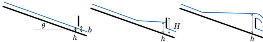
Figure 3: Flow modes for a leaky barrier.
