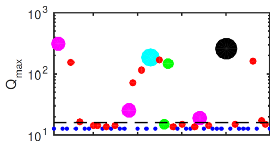
10 Figure 8 Maximum discharge at the downstream node for an ensemble of runs (indexed along abscissa) on the one-dimensional network in figure 2c, forced by the same upstream inflow q(t) = q_0 + q_{max} \exp(-t^2/\sigma^2) , with q_0 = 1 \text{ m}^3\text{s}^{-1} , q_{max} = 15 \text{ m}^3\text{s}^{-1} , and \sigma = 2 \text{ h} . The size and colour of the dots indicates the number of dams that failed during each realisation, and the dashed line shows the peak discharge in the case that no dams are installed. Parameter values are as given in section 2.3 except with l = 1000 \text{ m} , S = 0.005 , and \lambda = 20 , together with b = 0.3 \text{ m} and H = 1.5 \text{ m} .
