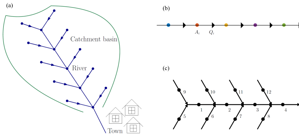
15 Figure 2: Schematic (a) and the 1d network (b) and 2d network (c) leaky barrier configurations investigated. Triangles indicate the location of dams which control the discharge, Q_i associated with the upstream reach where the average cross section is A_i .
