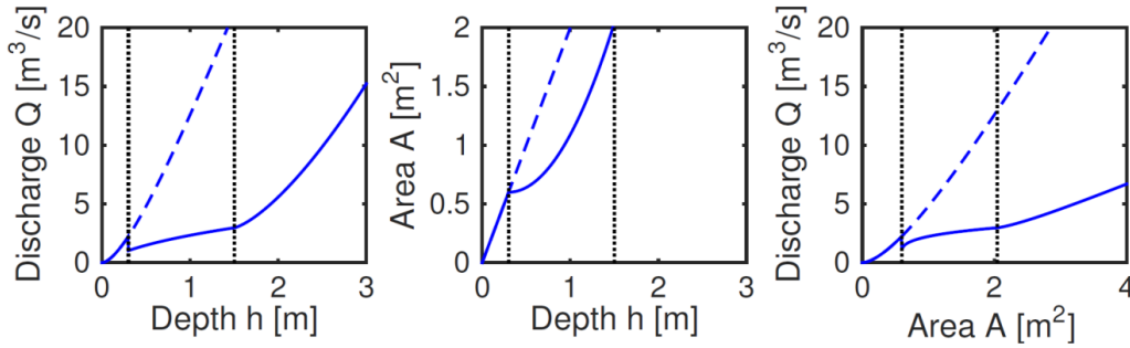
10 Figure 4: Examples of the relationships between discharge Q , cross-sectional area, A , and water depth h , for rectangular channel of width w=2\text{m} , slope S=0.01 , reach length l=100\text{m} , and Mannings n of 0.01 . Dashed lines show the case of no dam. Solid lines show cases of b=0.3\text{m} , H=1.5\text{m} , shown by the vertical dotted lines.
