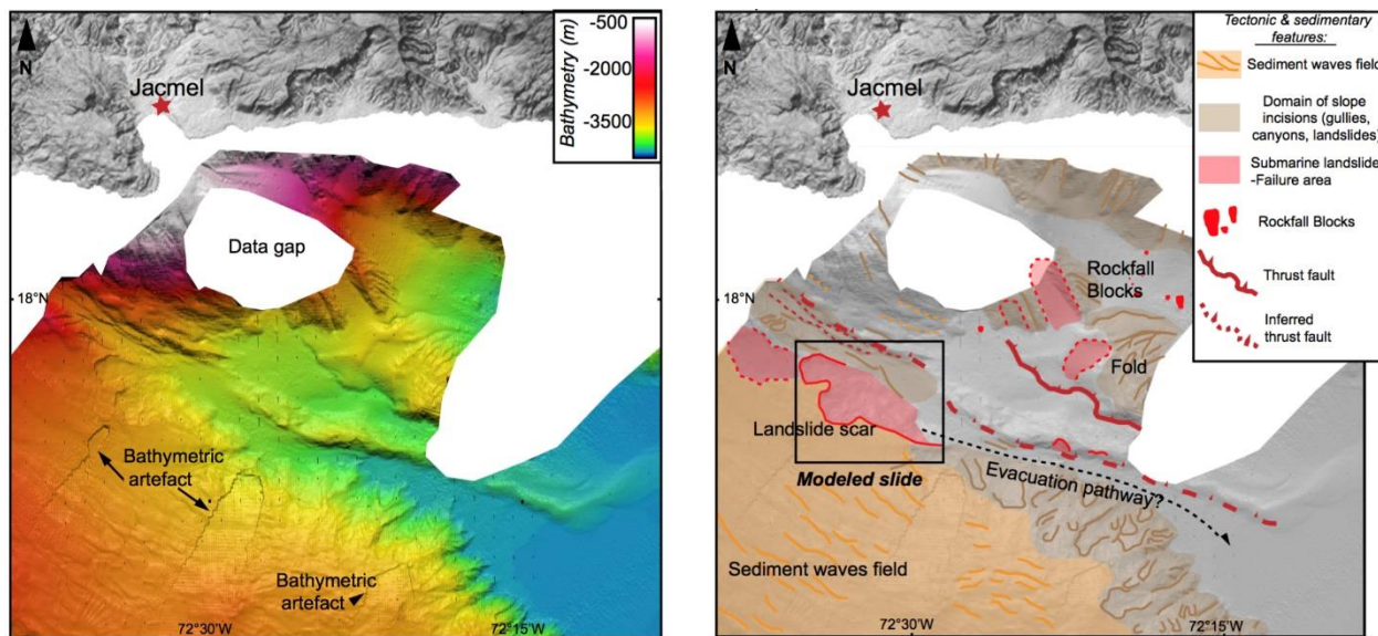
Figure 5: Detailed bathymetry 20 km due south of Jacmel (Fig. 1) where the landslide scar discussed in the text has been identified. Left: raw observations. Right: geological interpretation. Swath bathymetric data are from Haiti-sis cruise ( http://dx.doi.org/10.17600/12010070 ).
